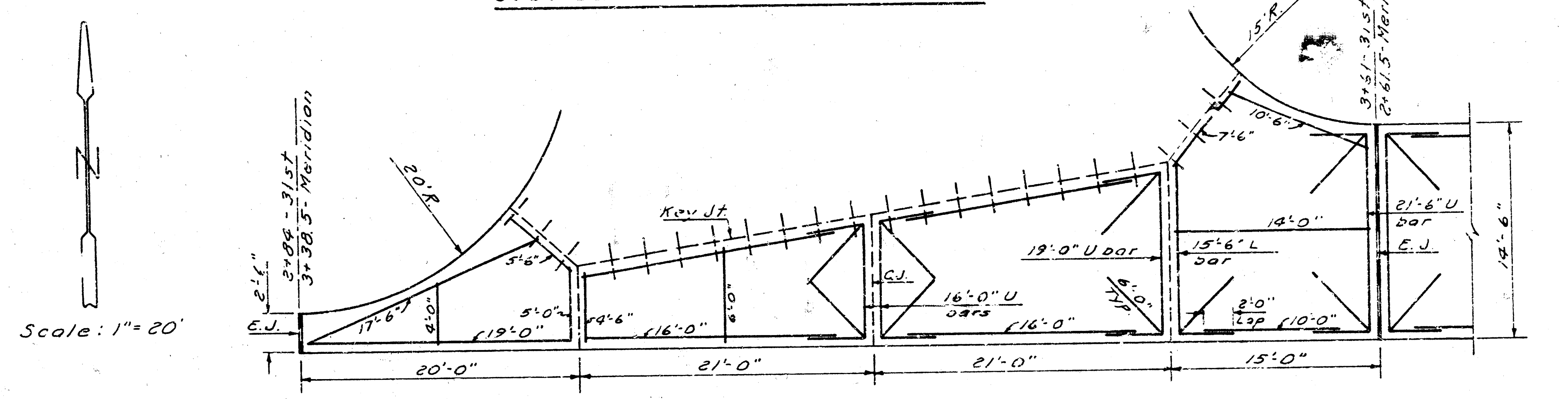
ENTRANCES STEEL PATTERN
