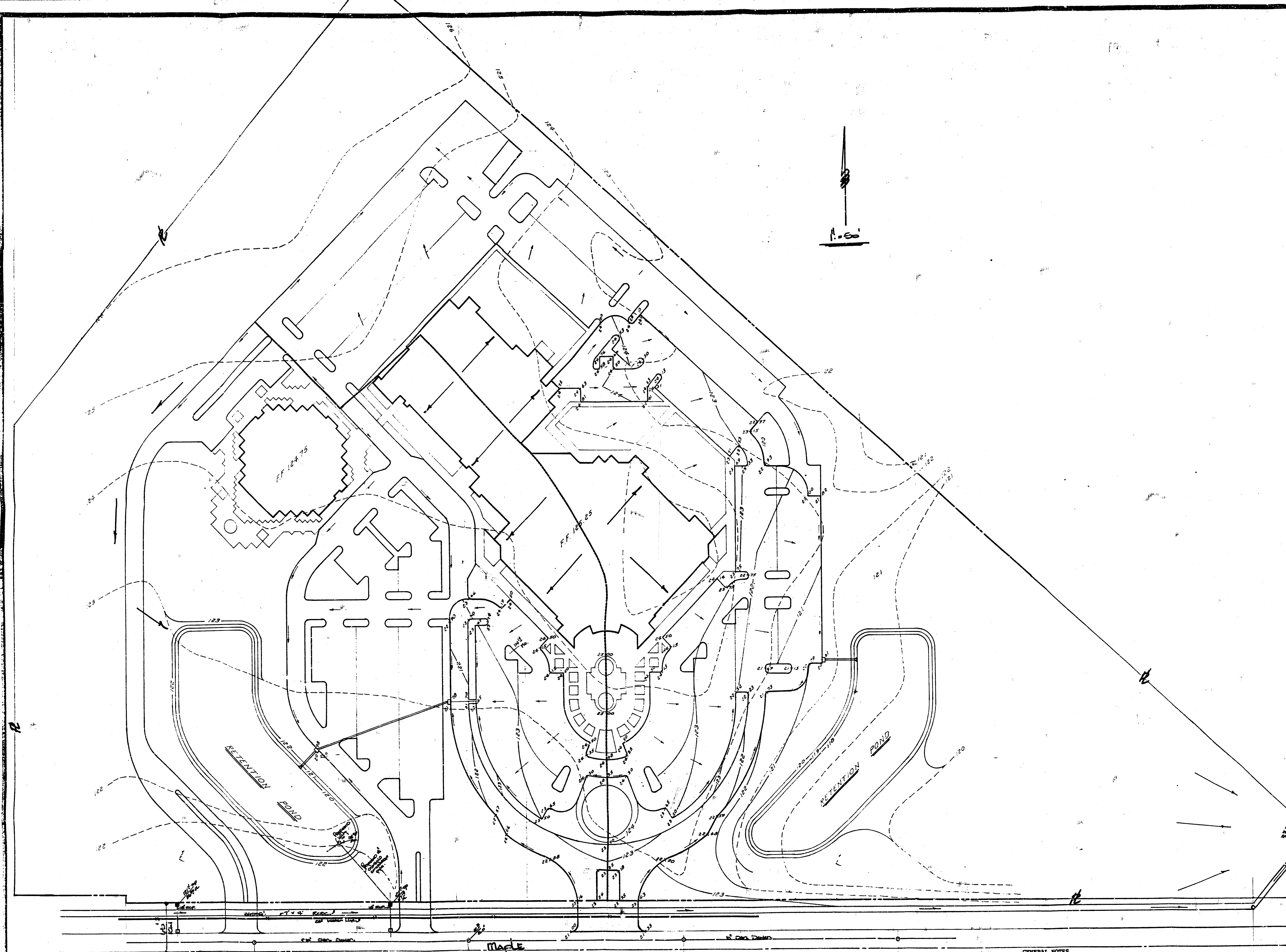
ANDRIA ADDITION DRAINAGE PLAN
