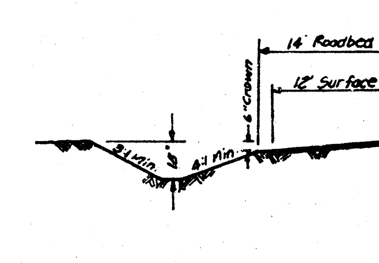
Note: Recommended Culvert Size for Drives are 12" @ 0.3%, Q=1.9 cfs.
