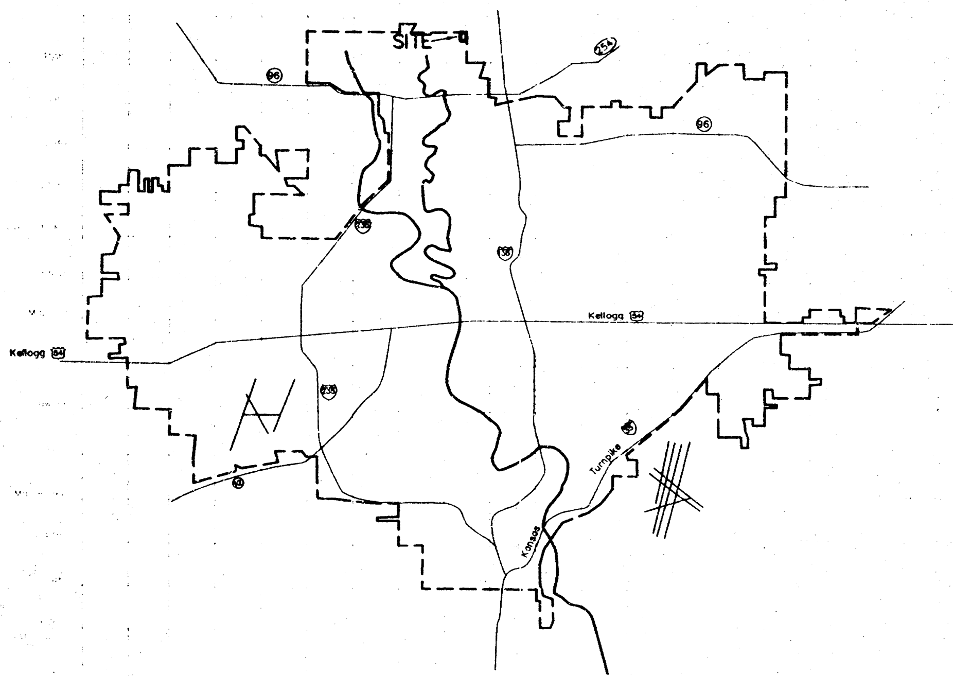
VICINITY MAP
