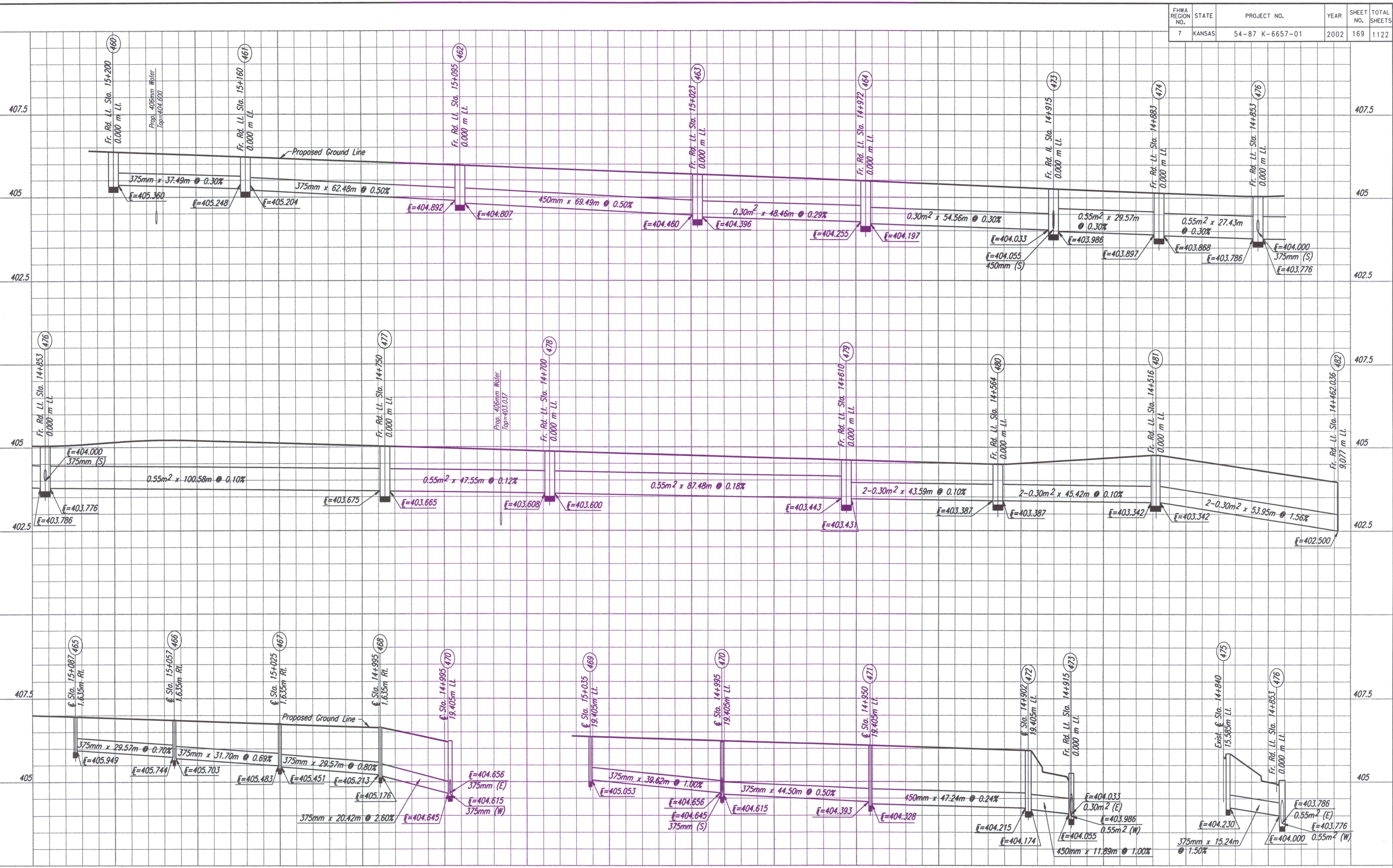
Storm Sewer Profiles Nodes 460-482
