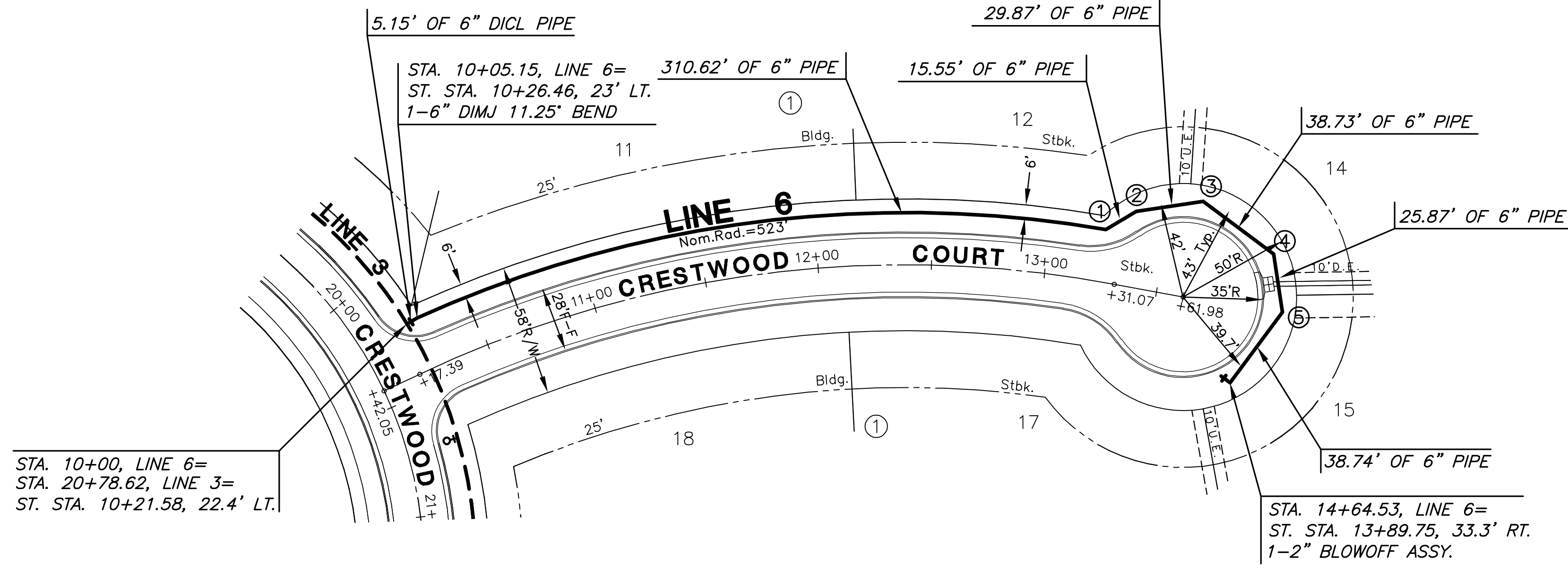
PLAN LINE 6
