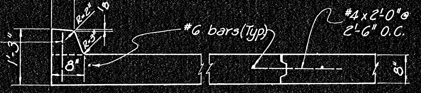
SECTION B-B
