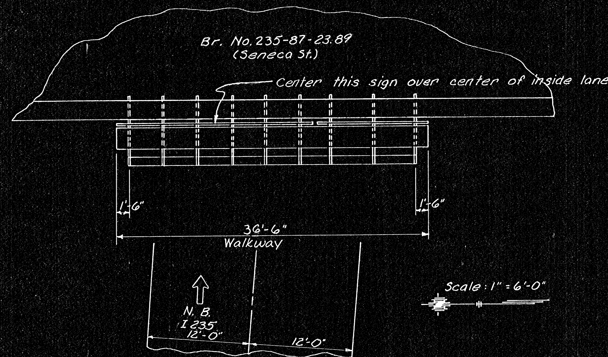
PLAN
