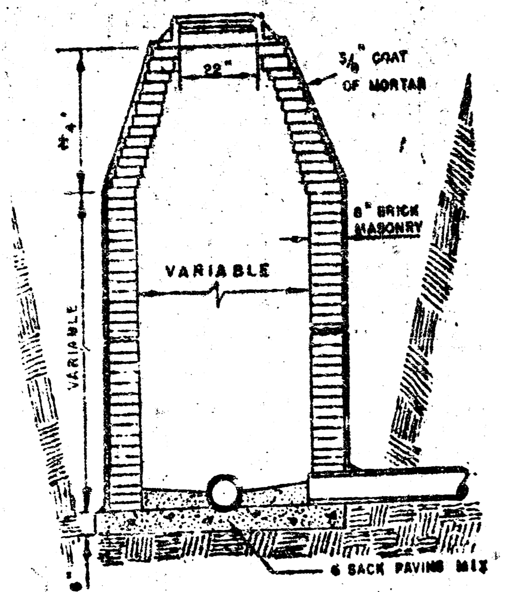
STANDARD MANHOLE TYPE "A" * 4' ON 5' DIA. M.H.
