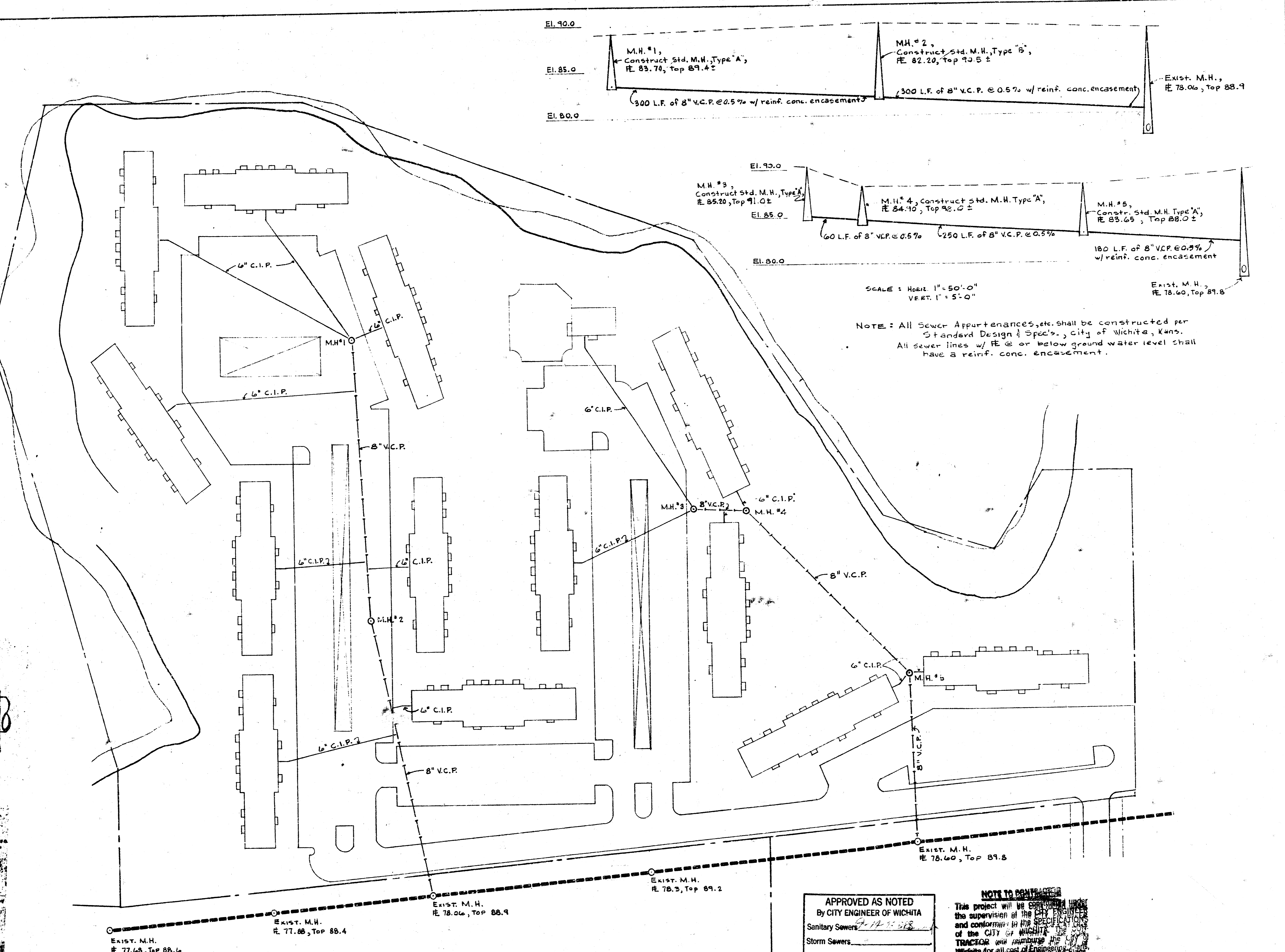
UTILITY PLAN SCALE: 1" = 50'-0"
