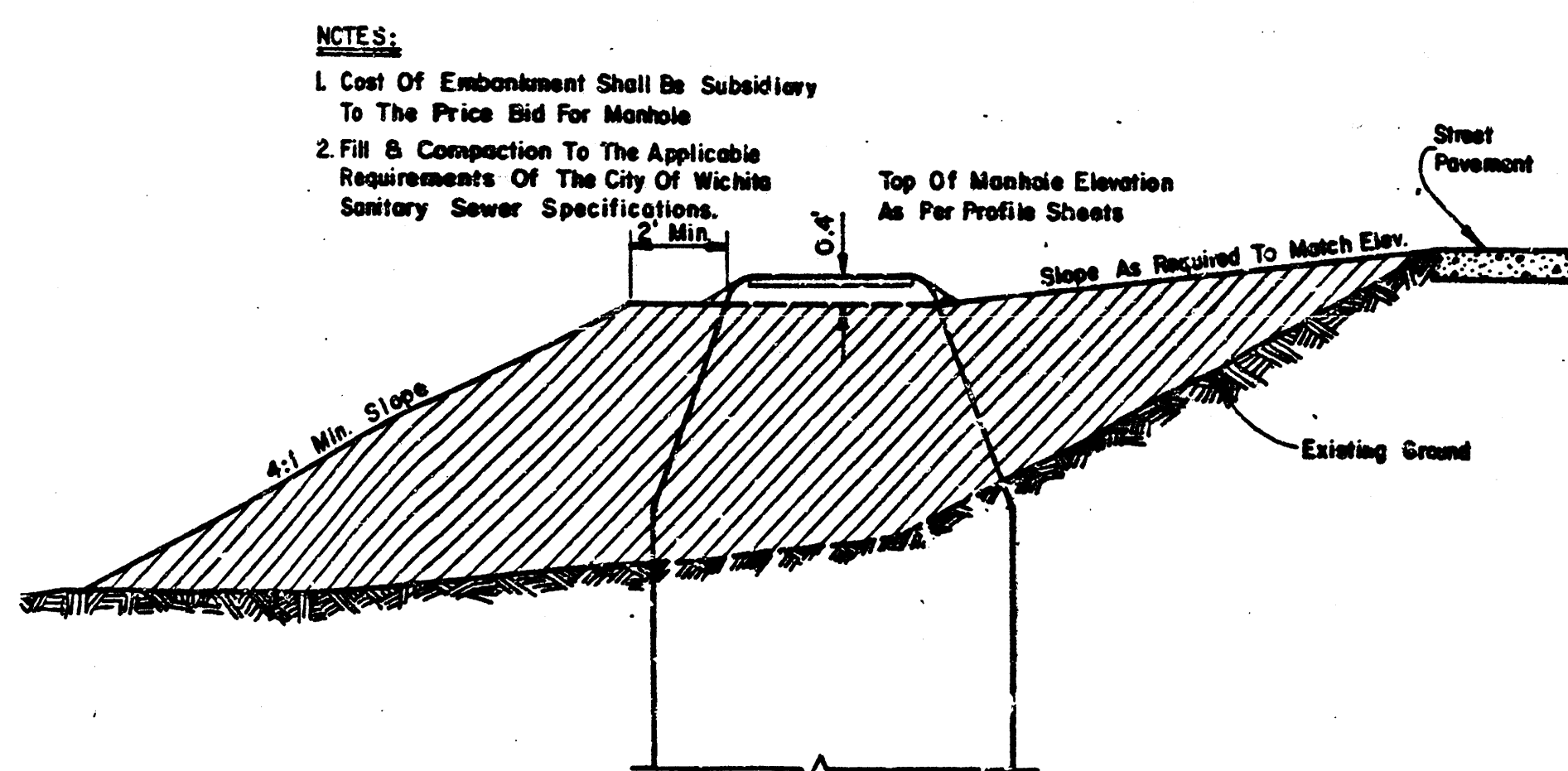
TYPICAL EMBANKMENT AROUND MANHOLE
