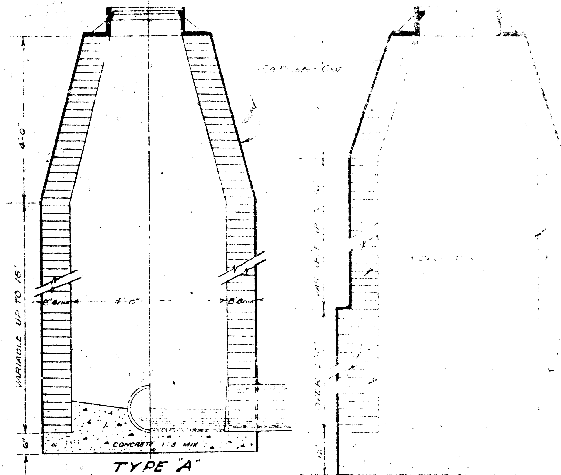
VERTICAL CROSS-SECTION OF MANHOLE SCALE 1/2"=1'-0"
