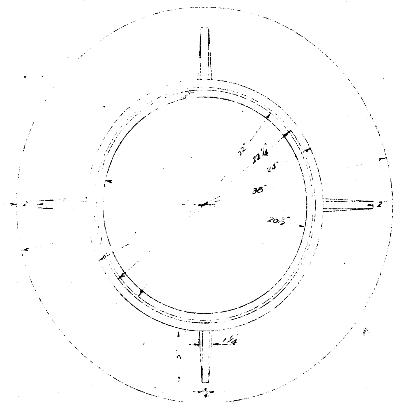
PLAN VIEW OF MANHOLE RING SCALE 1"=1'-0"
