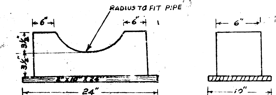
DETAIL OF CRADLE BLOCK
