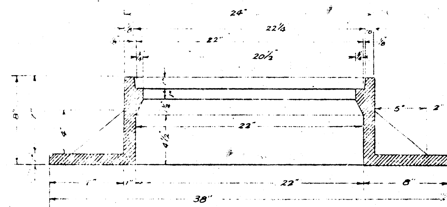
VERTICAL CROSS-SECTION OF MANHOLE RING SCALE 1"=1'-0"
