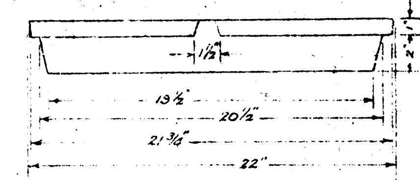
SIDE VIEW OF MANHOLE COVER SCALE 1"=1'-0"
