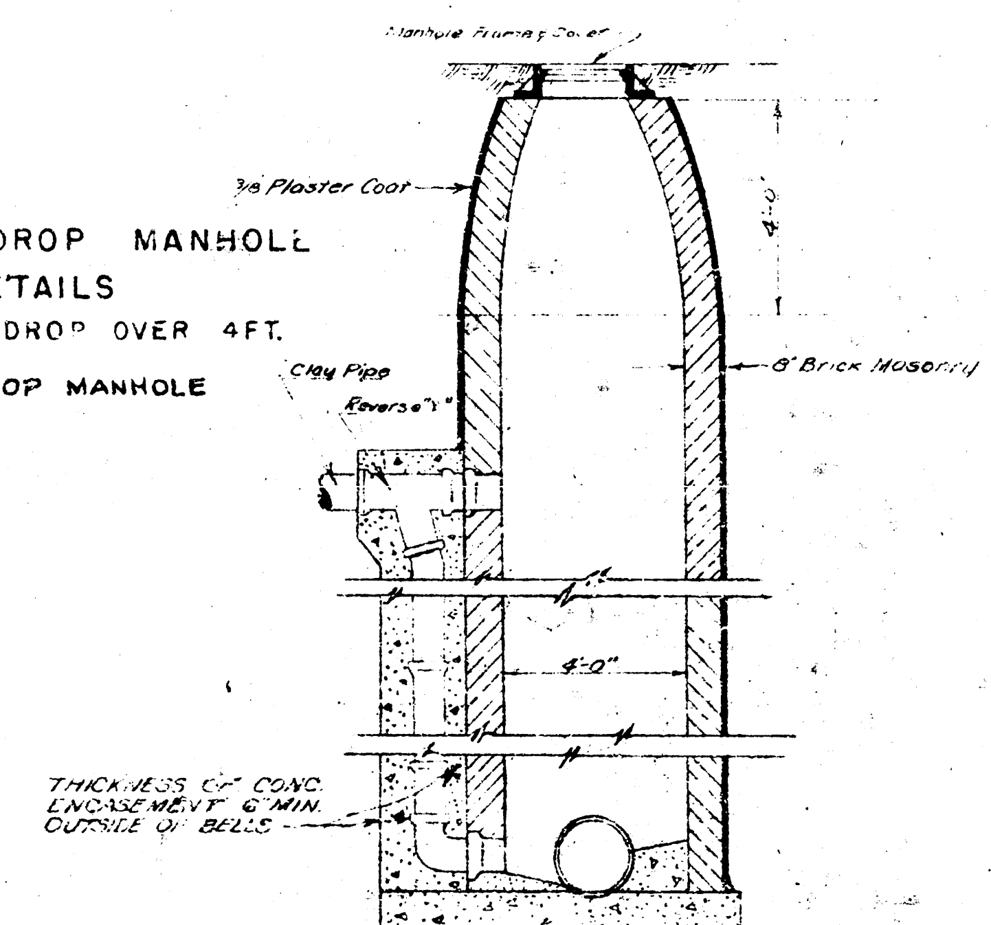
VERTICAL SECTION SCALE 1"=1'-0"
