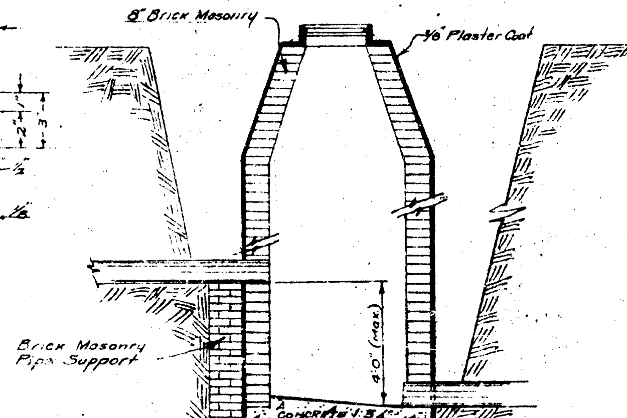
CROSS-SECTION OF DROP MANHOLE SCALE 1/2"=1'-0"
