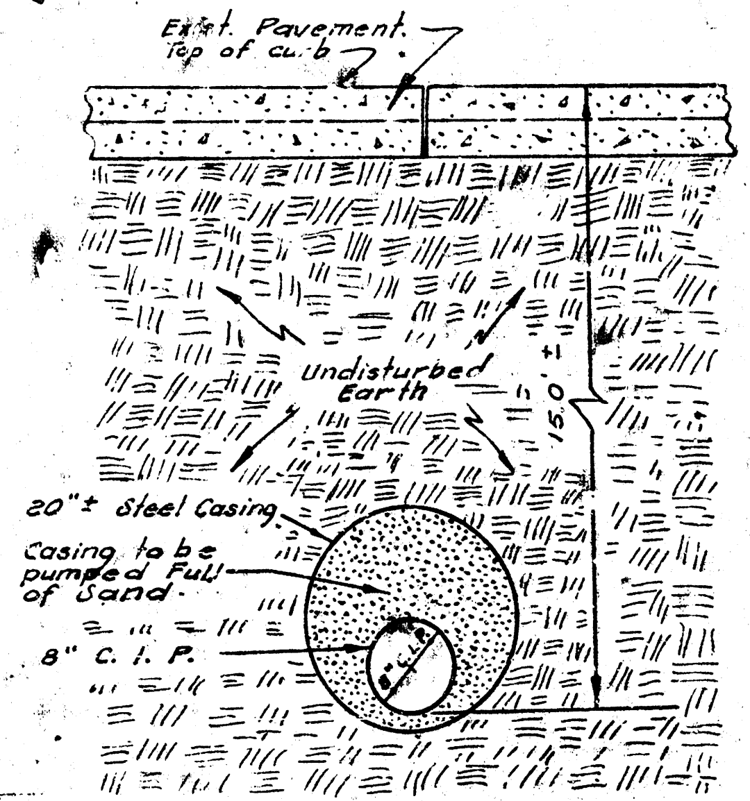
TYPICAL SECTION TUNNEL AT OLIVER ST. AND 31ST ST. SO. Sta. 3115.0 to Sta. 3185.0 SCALE 1" = 2'
