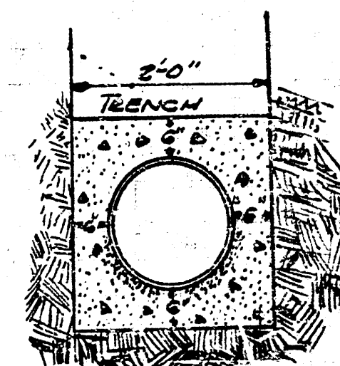
CONCRETE ENCASMENT DETAIL NO SCALE
