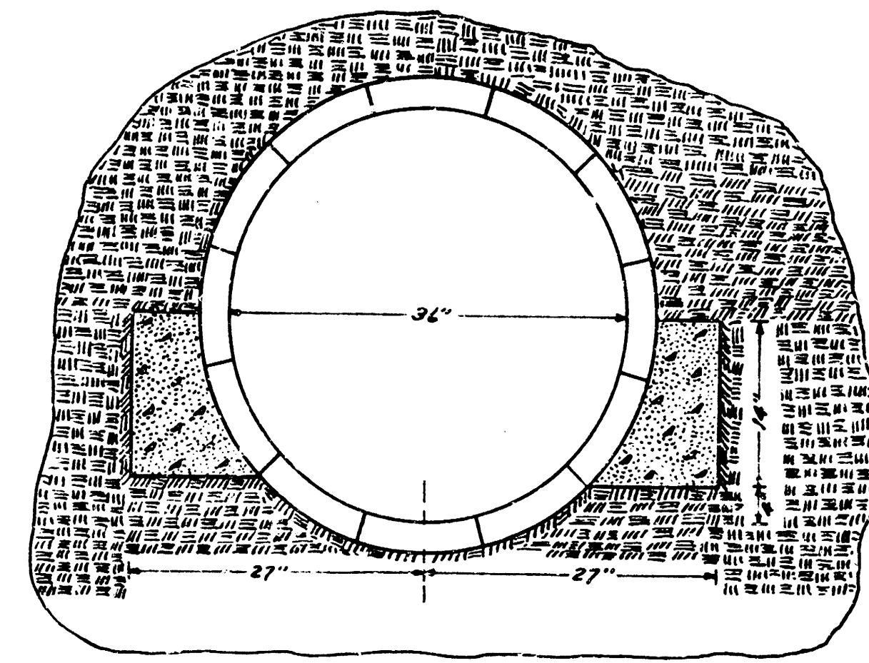
CONCRETE CRADLE FOR SEGMENT BLOCK SEWER Scale 1/4" = 1'-0"
