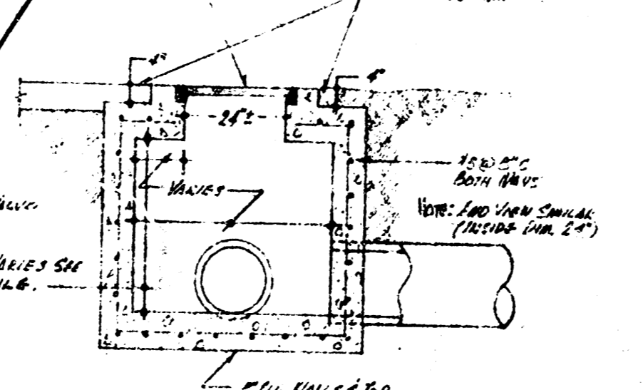
TYPICAL SECTION THRU CATCH BASIN SCALE 1/4" = 1'-0"
