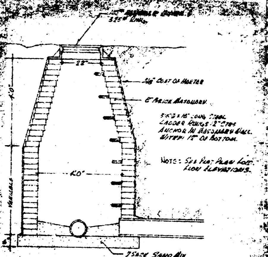
MANHOLE DETAIL NO SCALE
