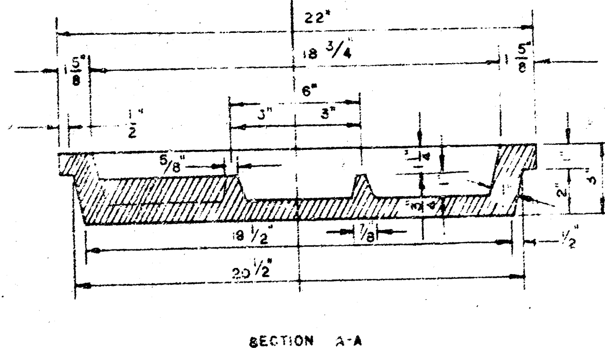
MANHOLE COVER
