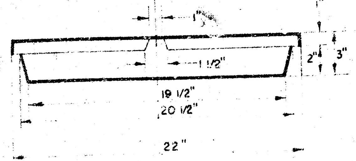
MANHOLE COVER
