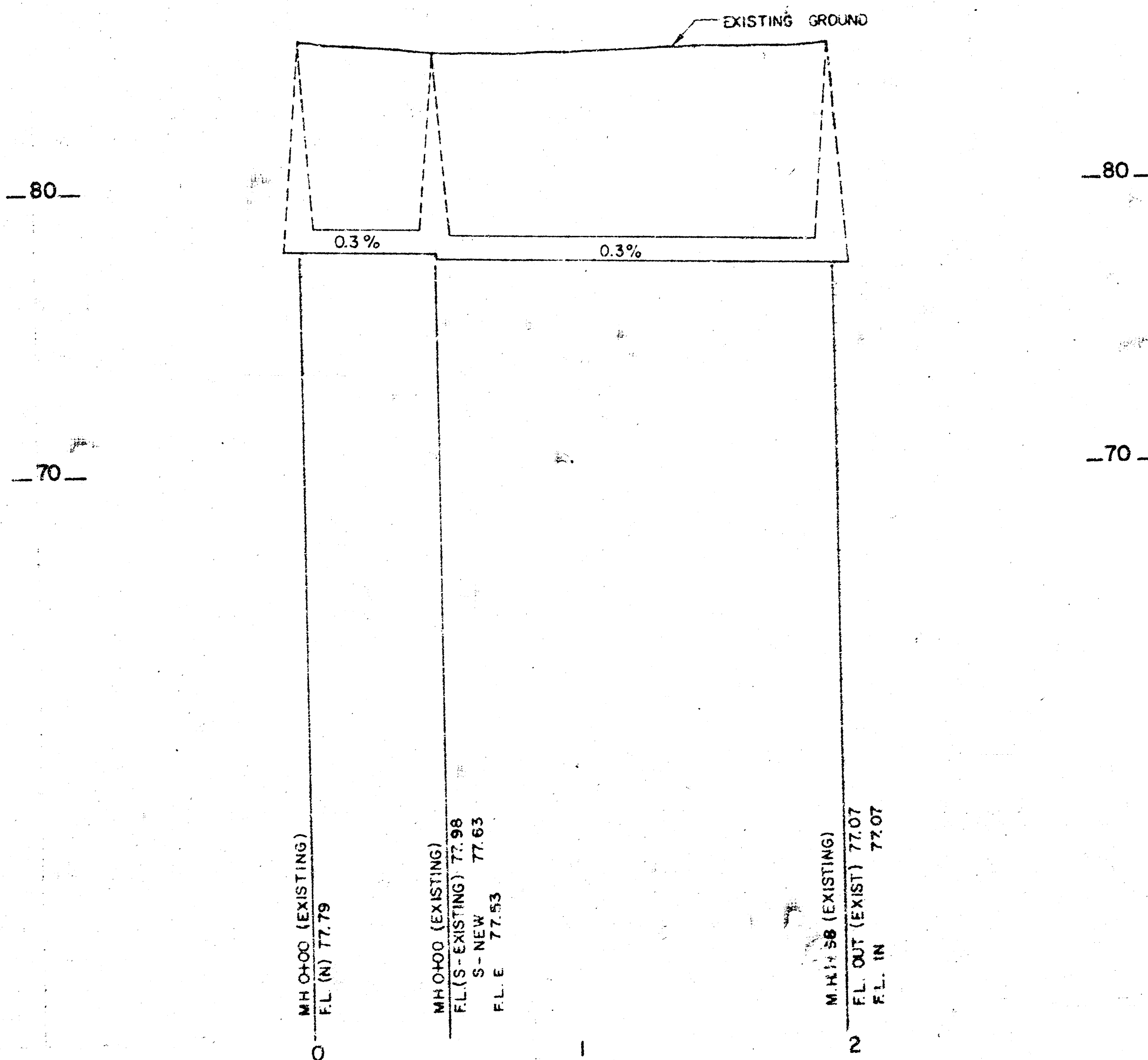
MAIN 1 EXTENSION ALL PIPE IS 8"
