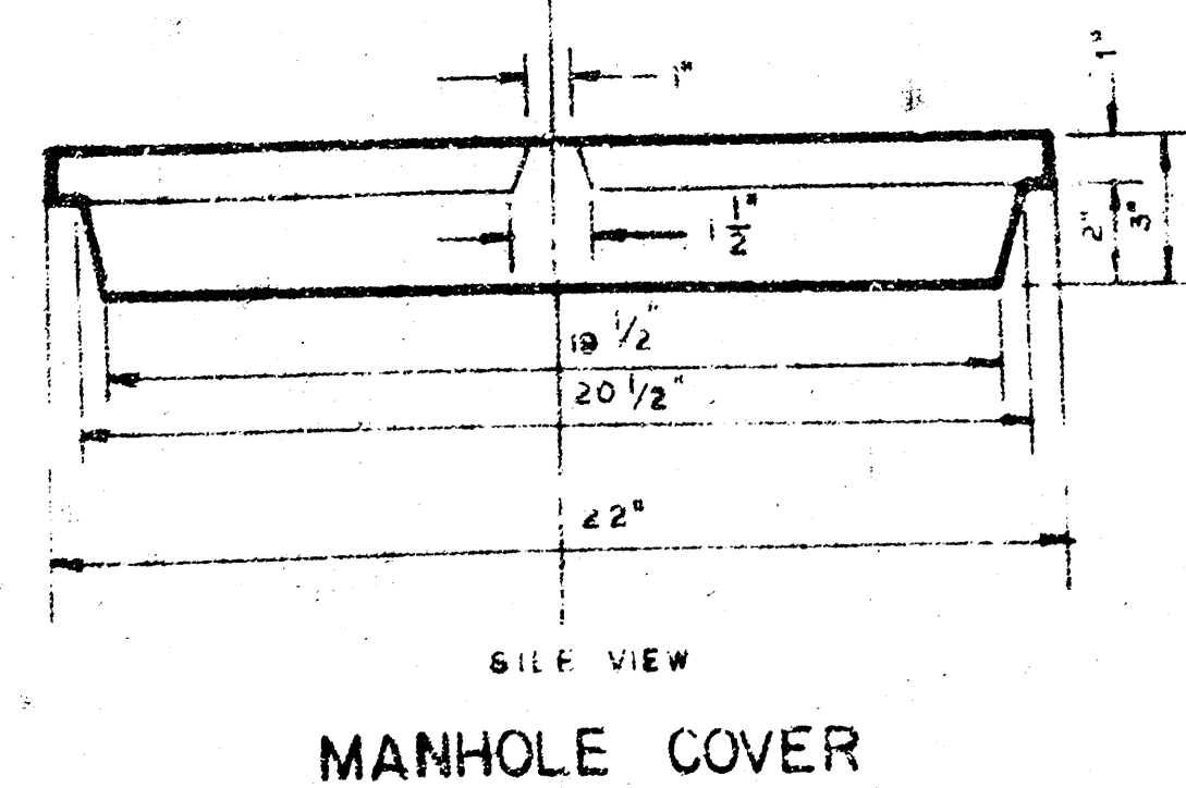
MANHOLE COVER
