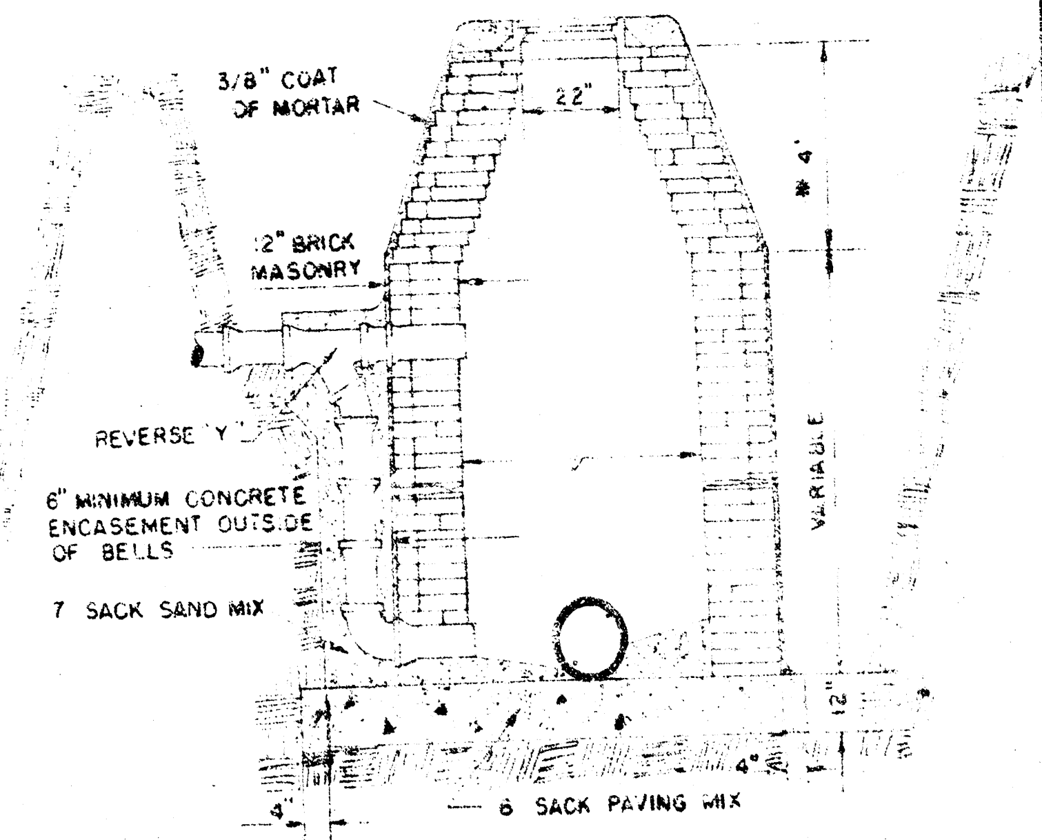
OUTSIDE DROP MANHOLE TYPE "B"
