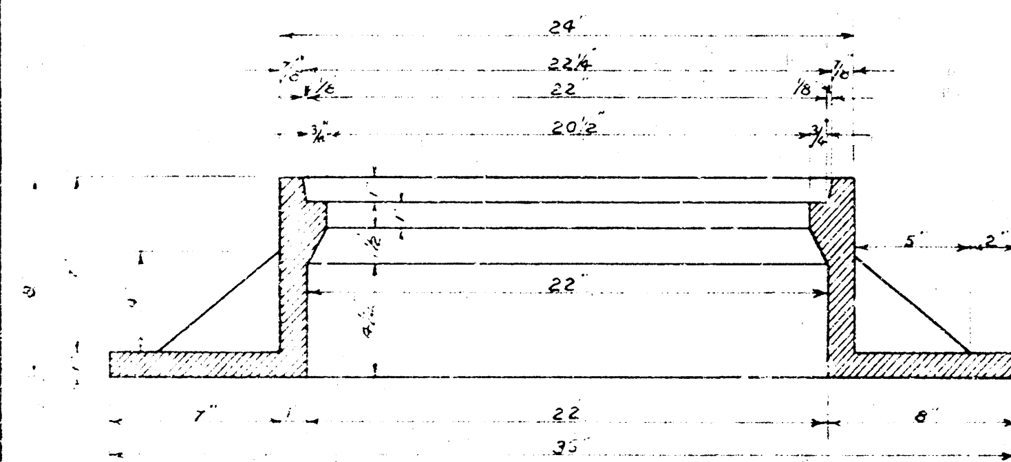
CROSS SECTION OF MANHOLE RING
