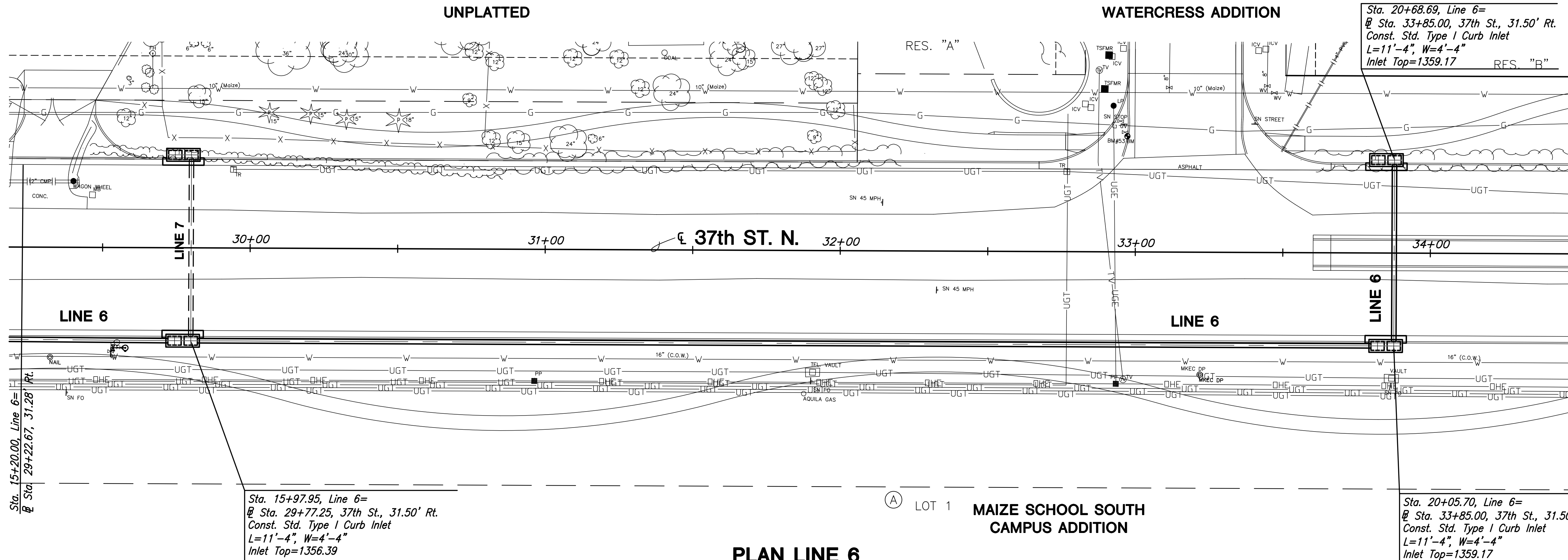
PLAN LINE 6 PROFILE LINE 6 SCALE: HORIZ. 1"=20' SCALE: VERT. 1"=5'
