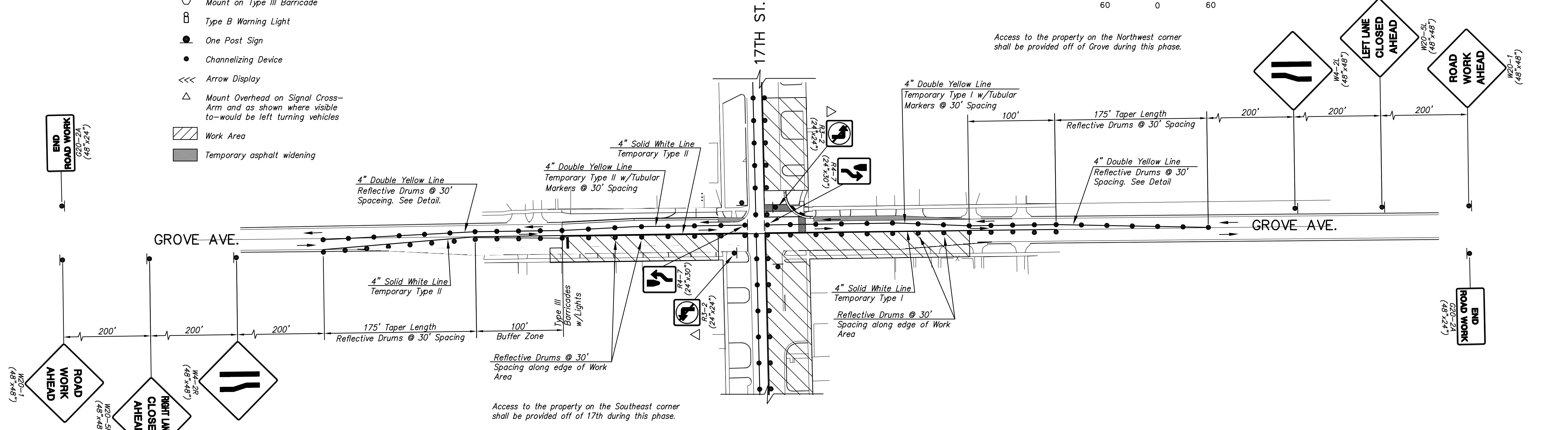
TRAFFIC CONTROL PLAN - PHASE 3
