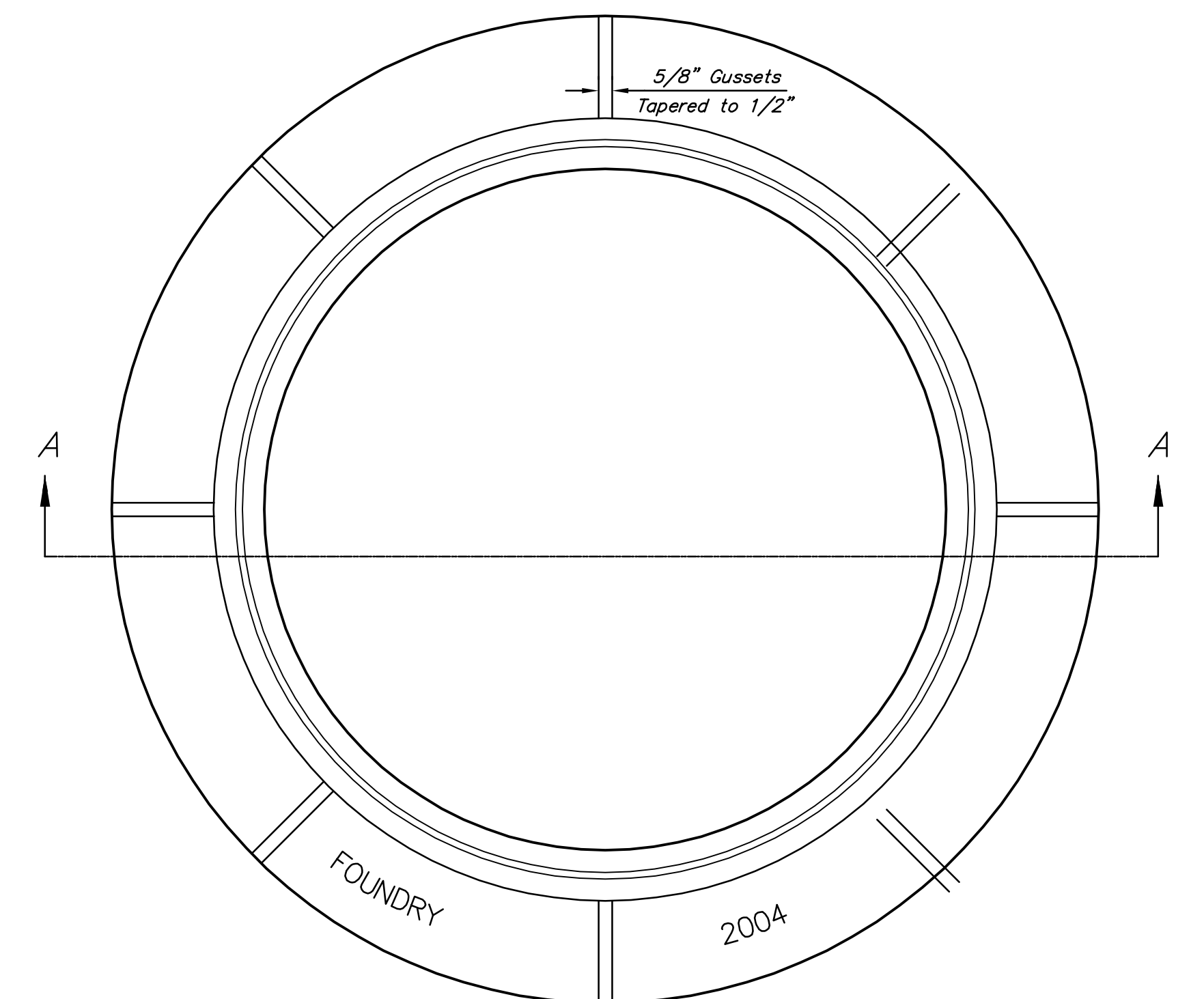
TOP VIEW
