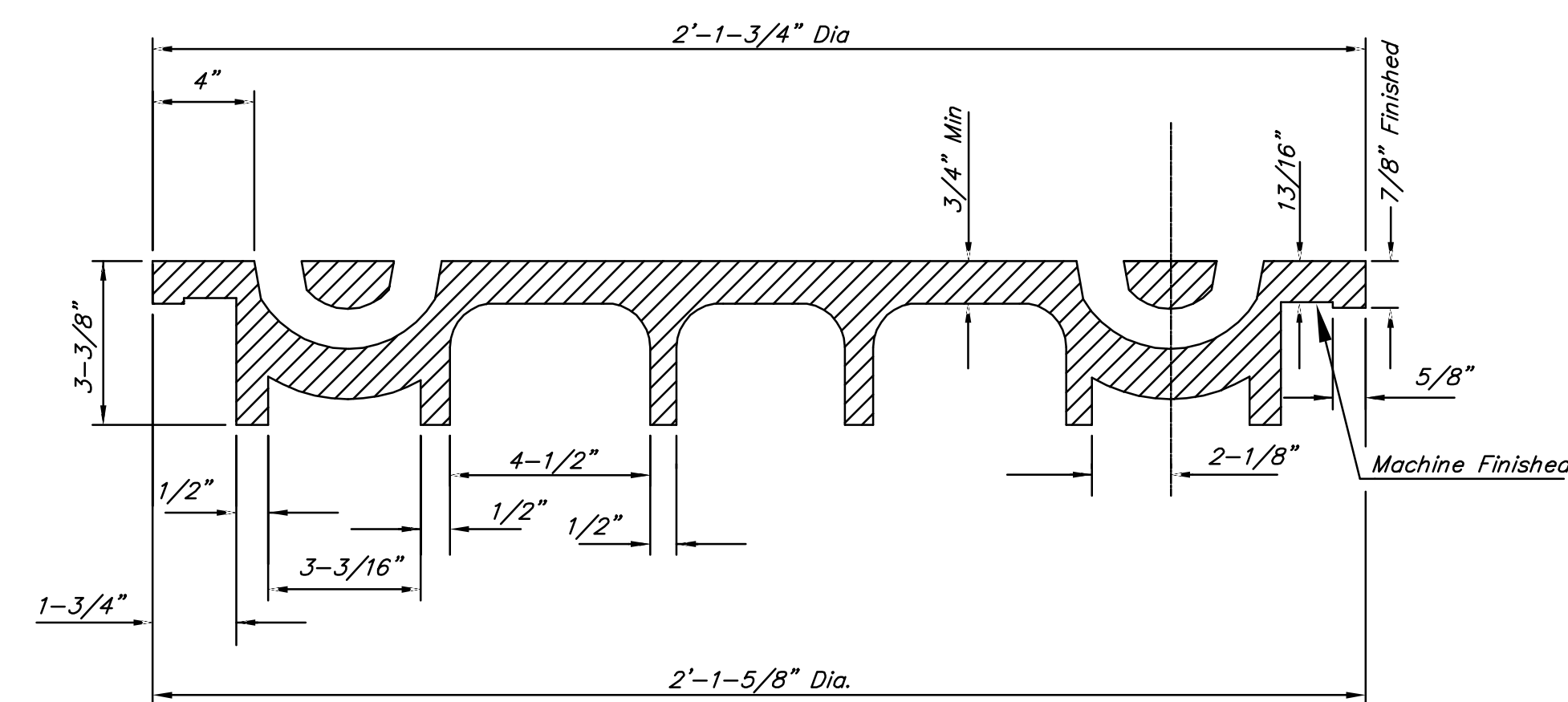
SECTION VIEW
