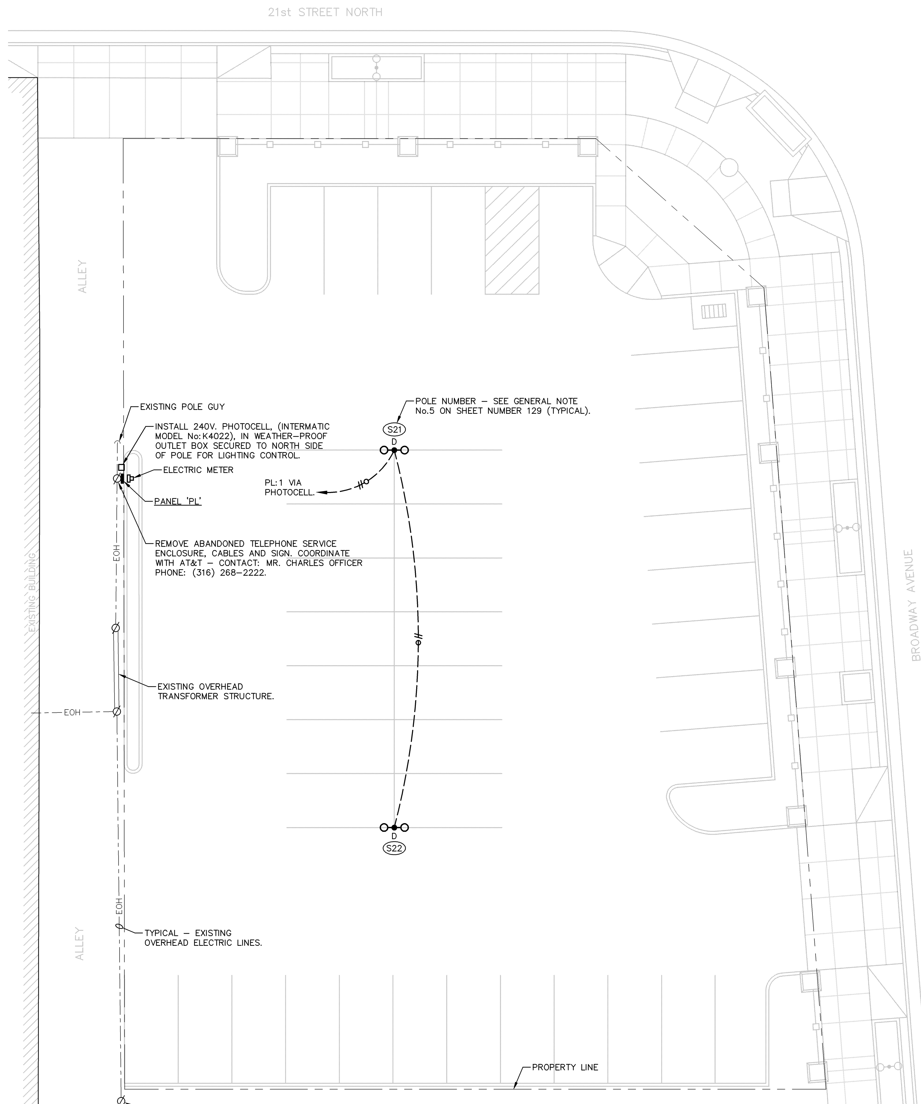
A PARKING LOT LIGHTING PLAN 1" = 10'-0"
