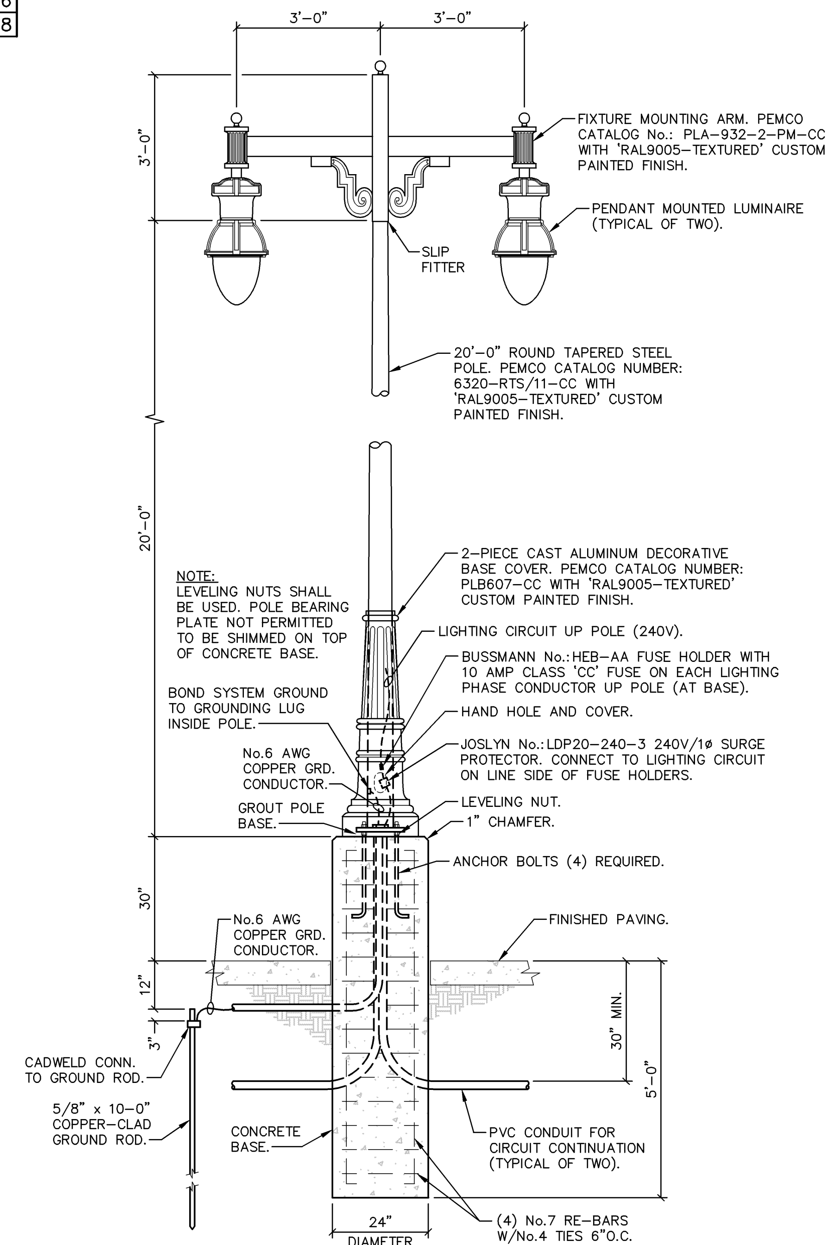
C LIGHTING POLE TYPE 'D' 1/2" = 1'-0"
