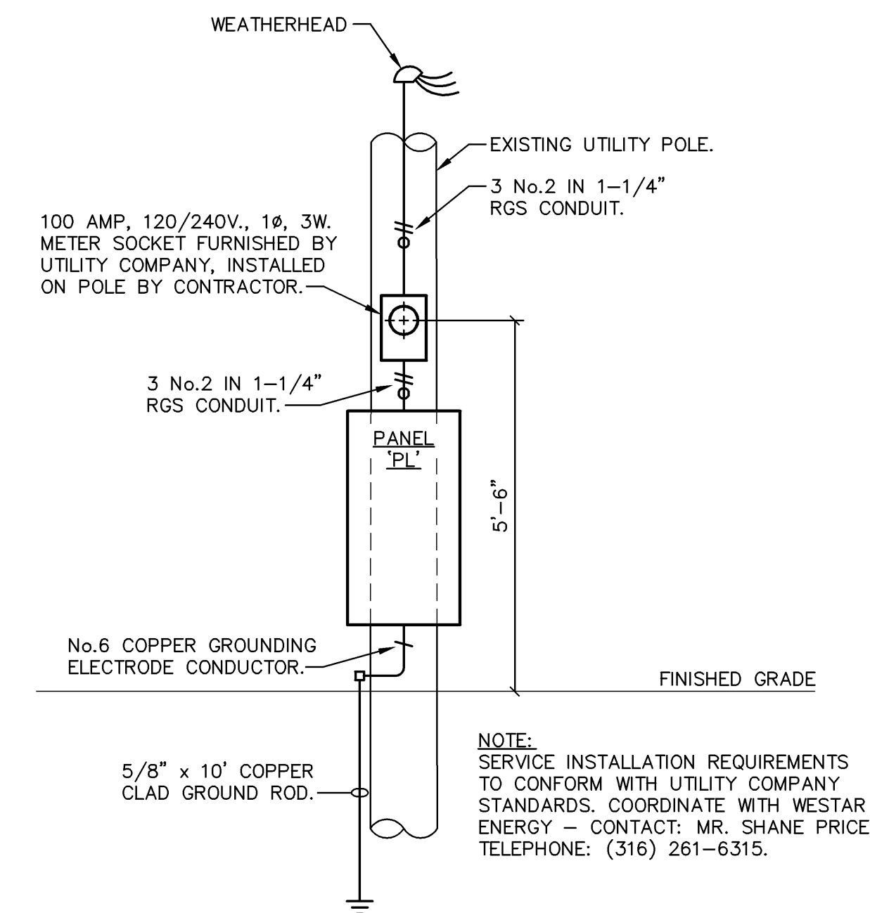
B PARKING LOT SERVICE BRISER DIAGRAM 1/2" = 1'-0"
