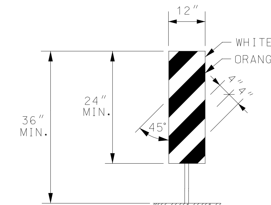
VERTICAL PANEL
