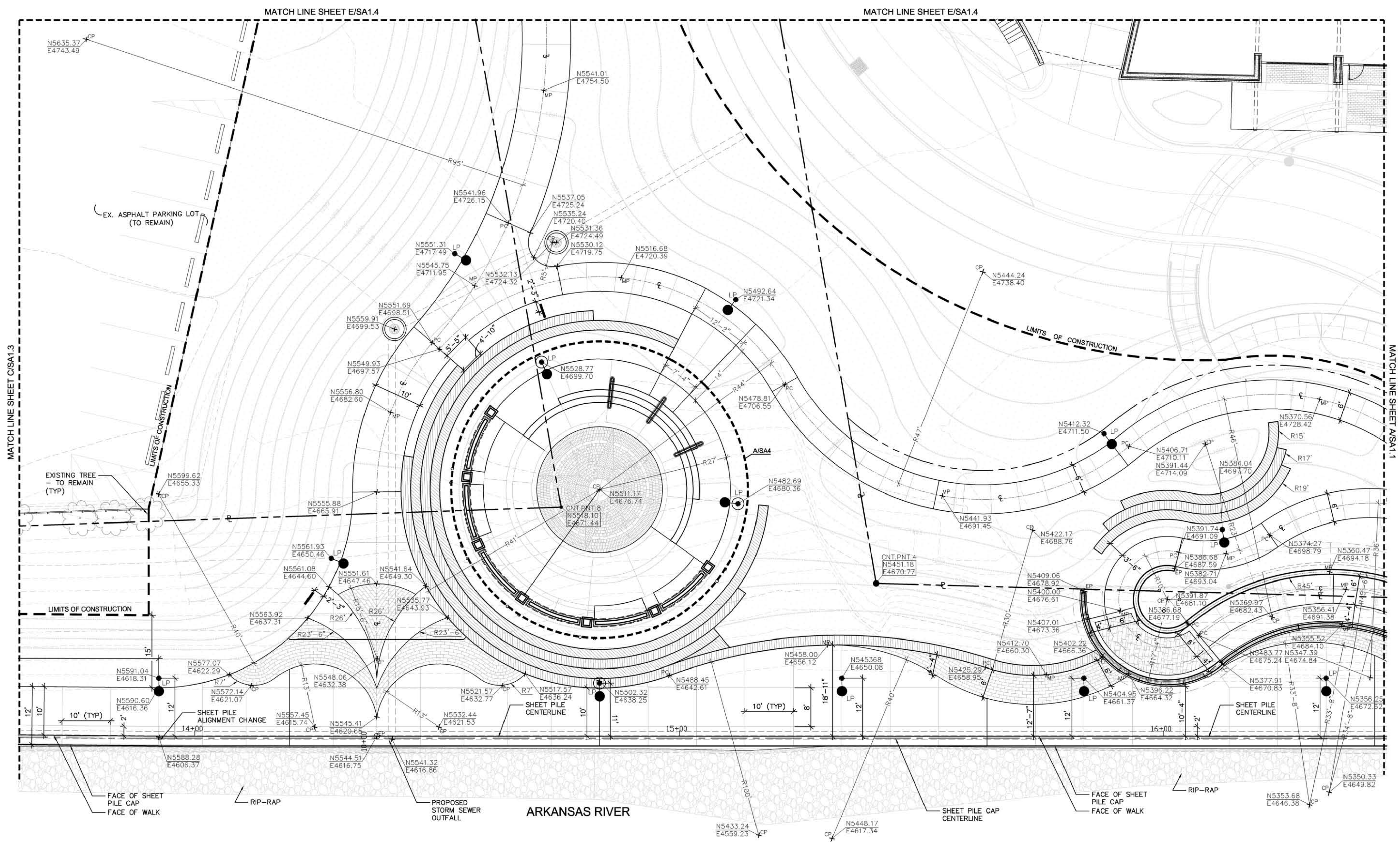
B SITE DIMENSION & LOCATION PLAN • SITE FINISHES & DETAIL CALL-OUTS REFER TO SA2 SHEETS • GRADING REFER TO SA3 SHEETS 1"=10'-0"
