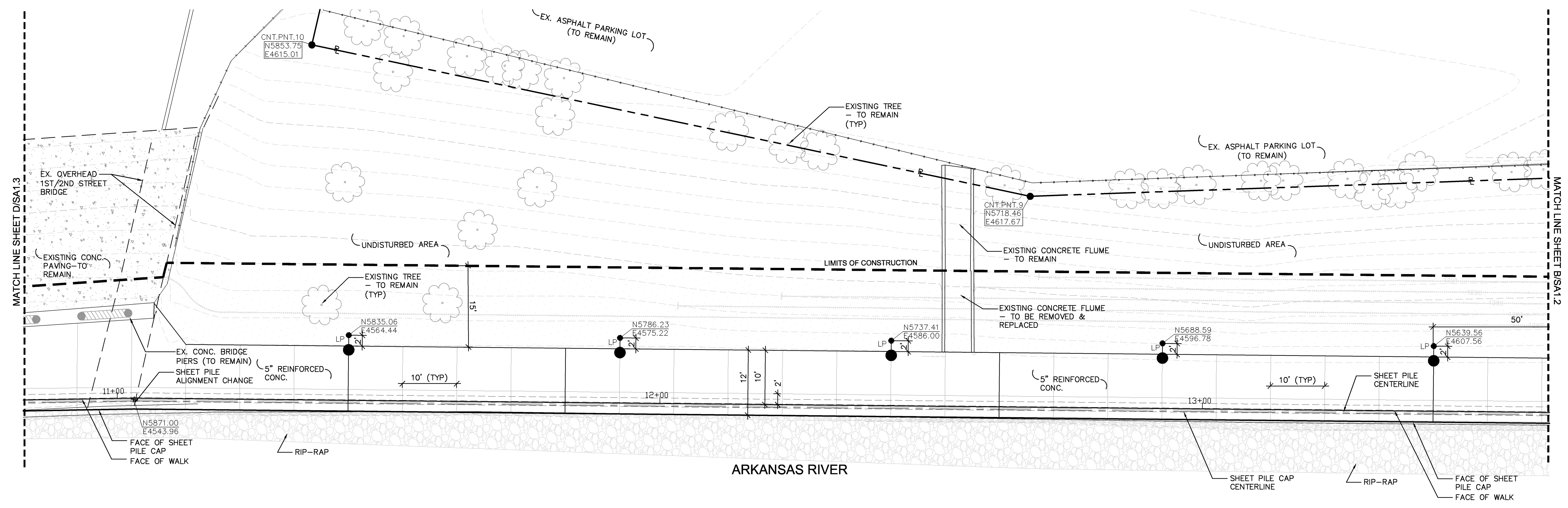
C SITE DIMENSION & LOCATION PLAN • SITE FINISHES & DETAIL CALL-OUTS REFER TO SA2 SHEETS • GRADING REFER TO SA3 SHEETS 1"=10'-0" NORTH
