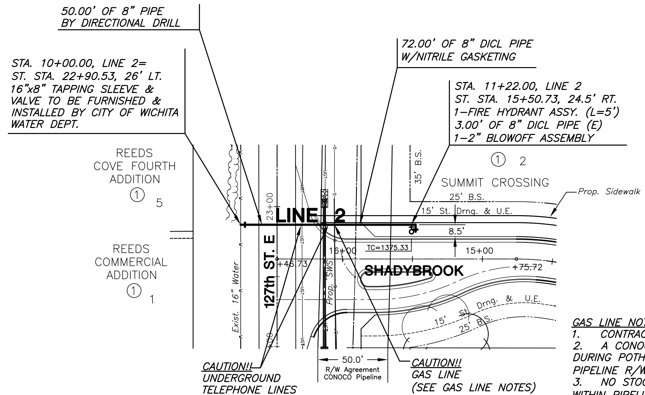
PLAN LINE 2
