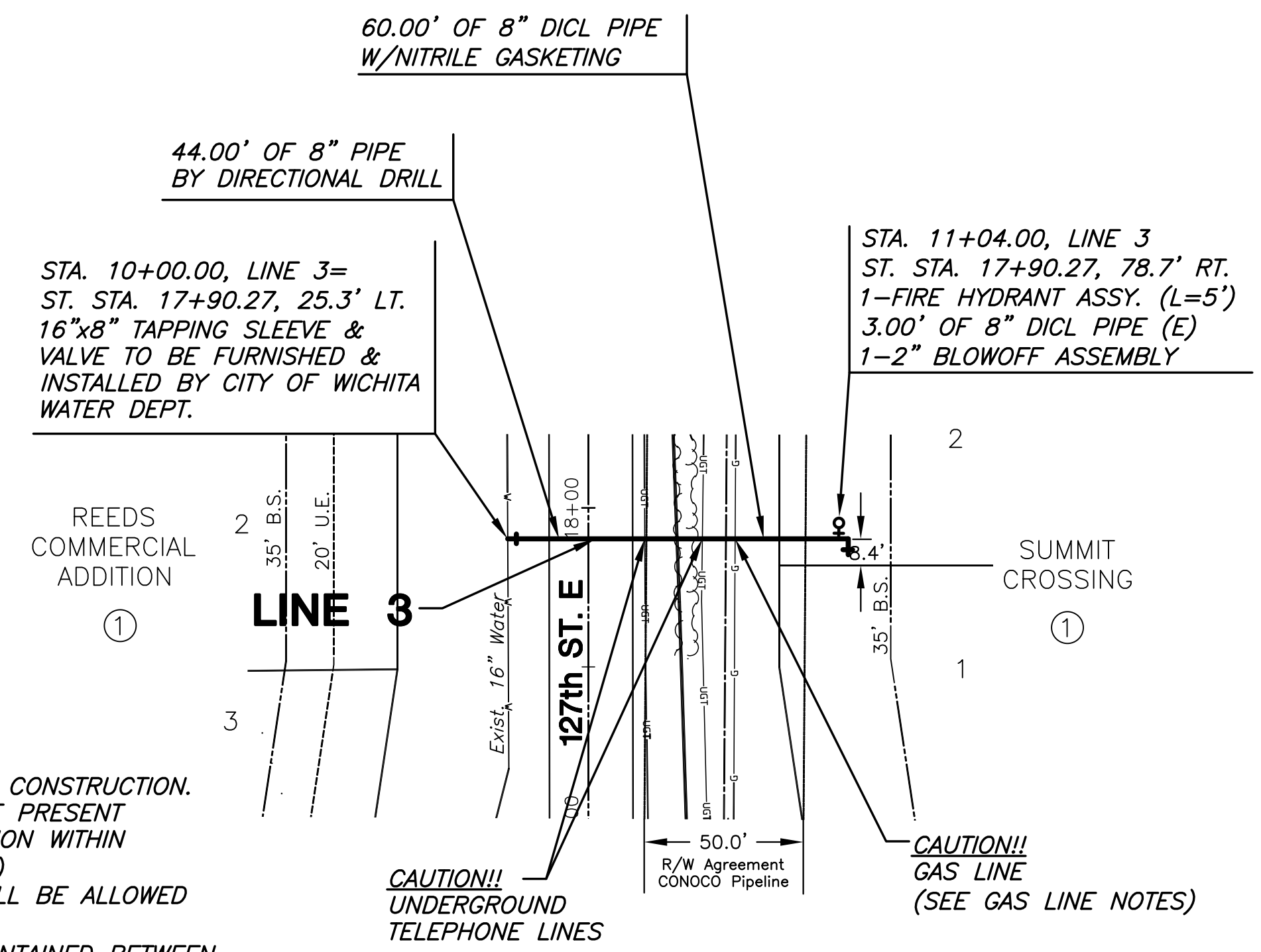
PLAN LINE 3
