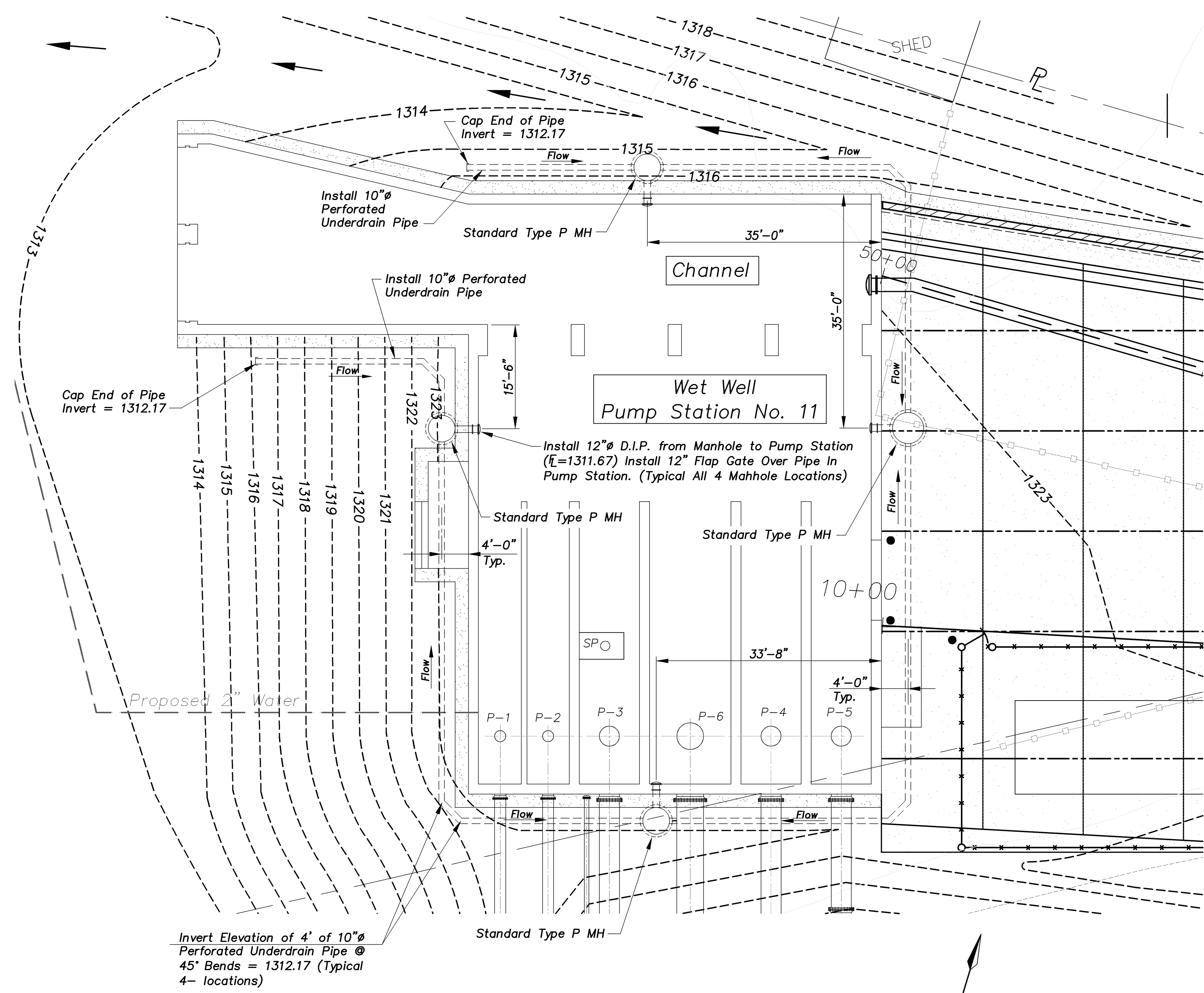
UNDERDRAIN PLAN
