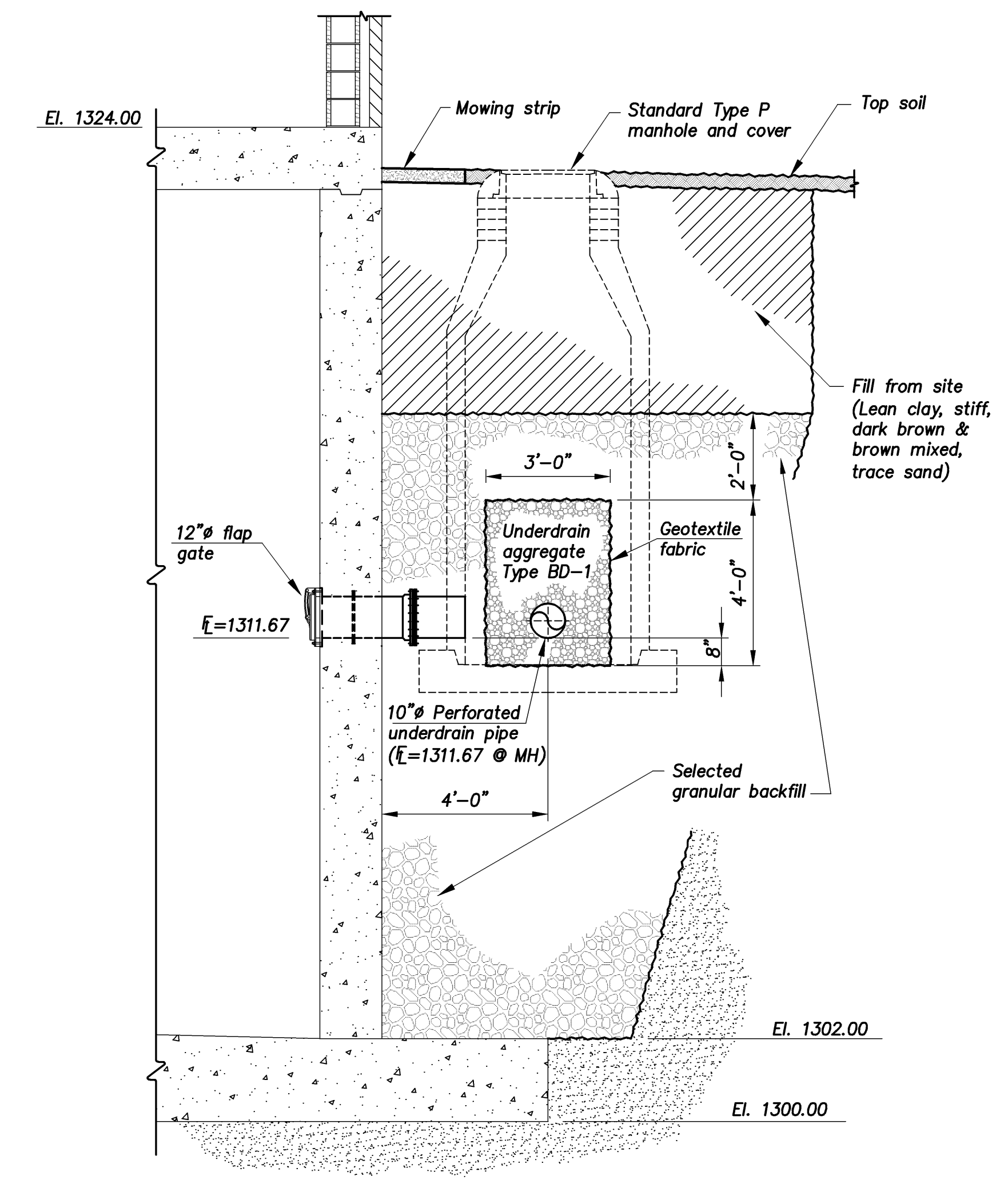
TYPICAL UNDERDRAIN SECTION Scale: 3/8" = 1'-0"
