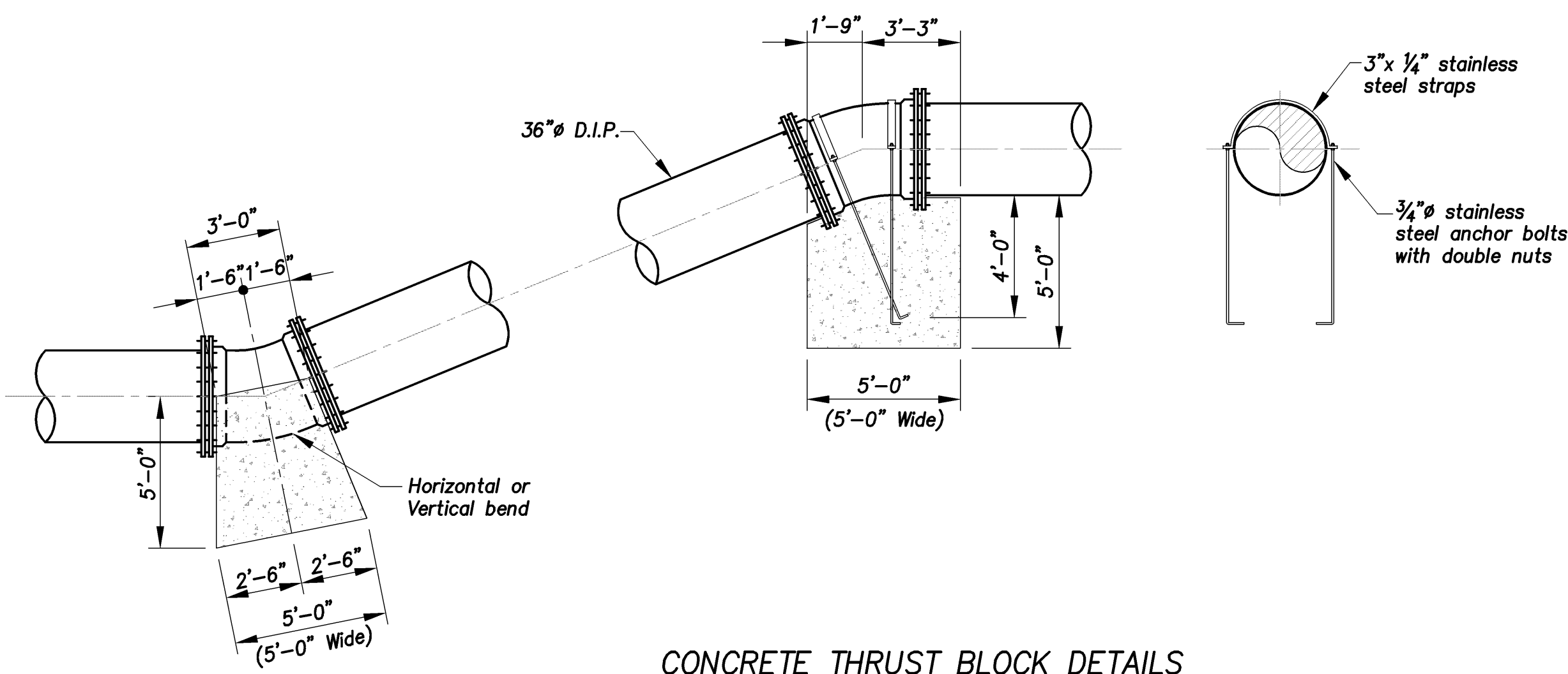
CONCRETE THRUST BLOCK DETAILS Scale: 1/4" = 1'-0"
