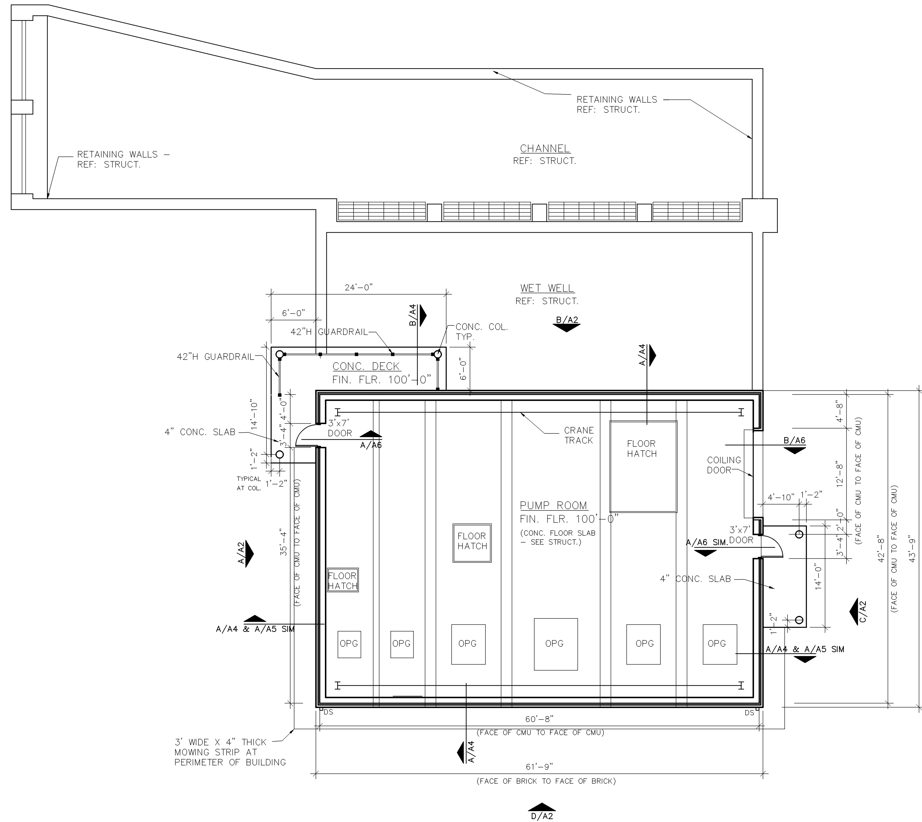
FLOOR PLAN 1/8" = 1'-0"
