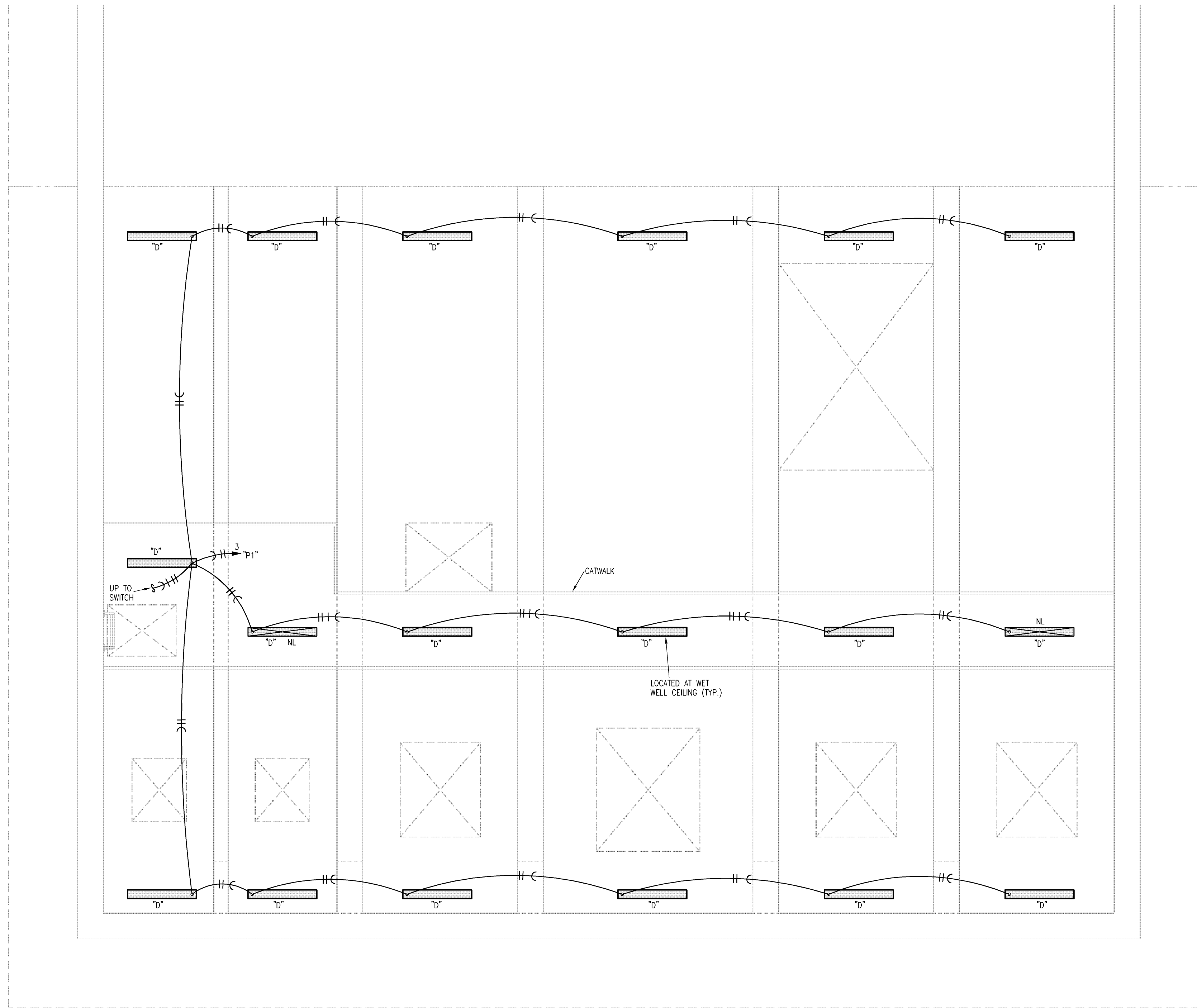
1 WET WELL PLAN 1/4"=1'-0" LIGHTING
