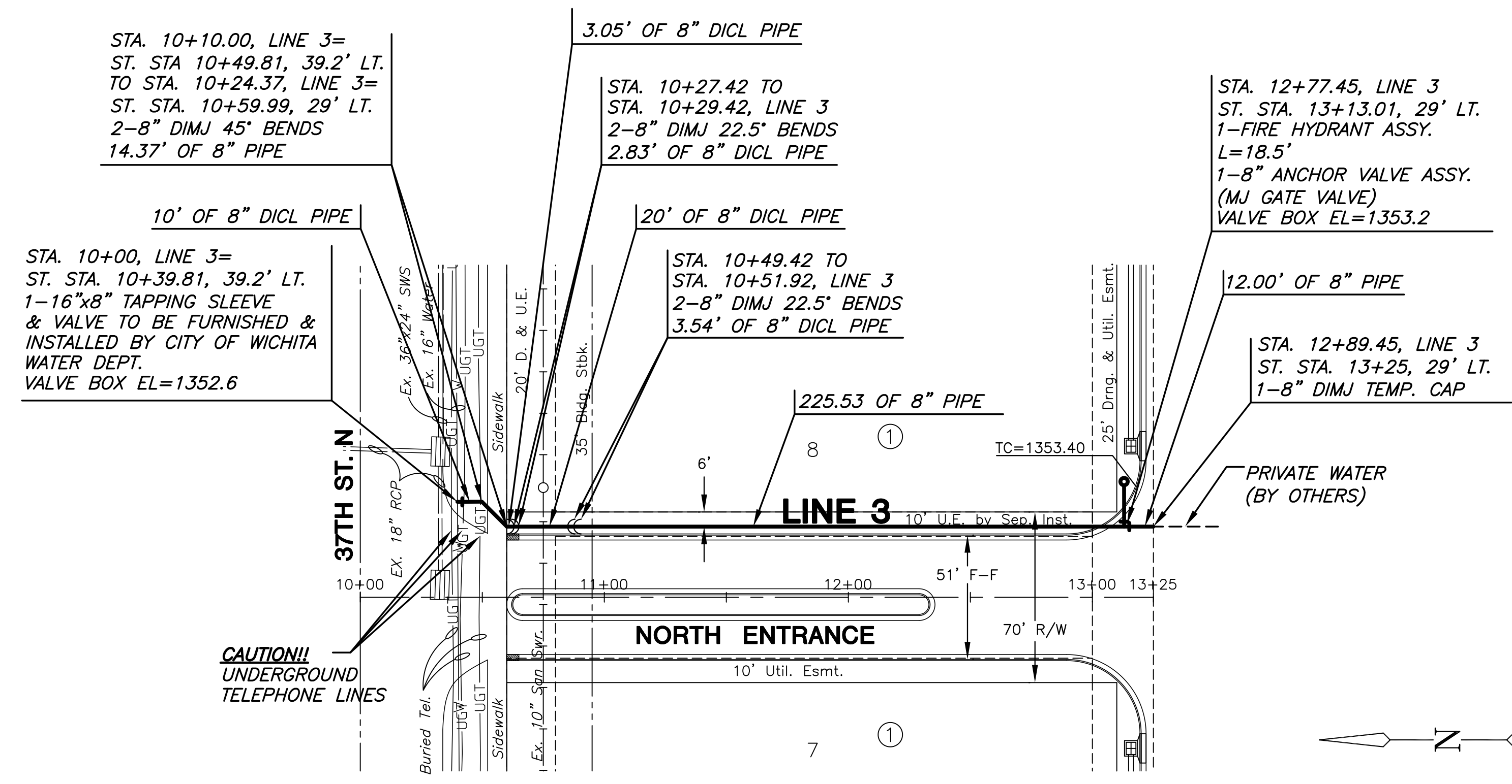
PLAN LINE 3
