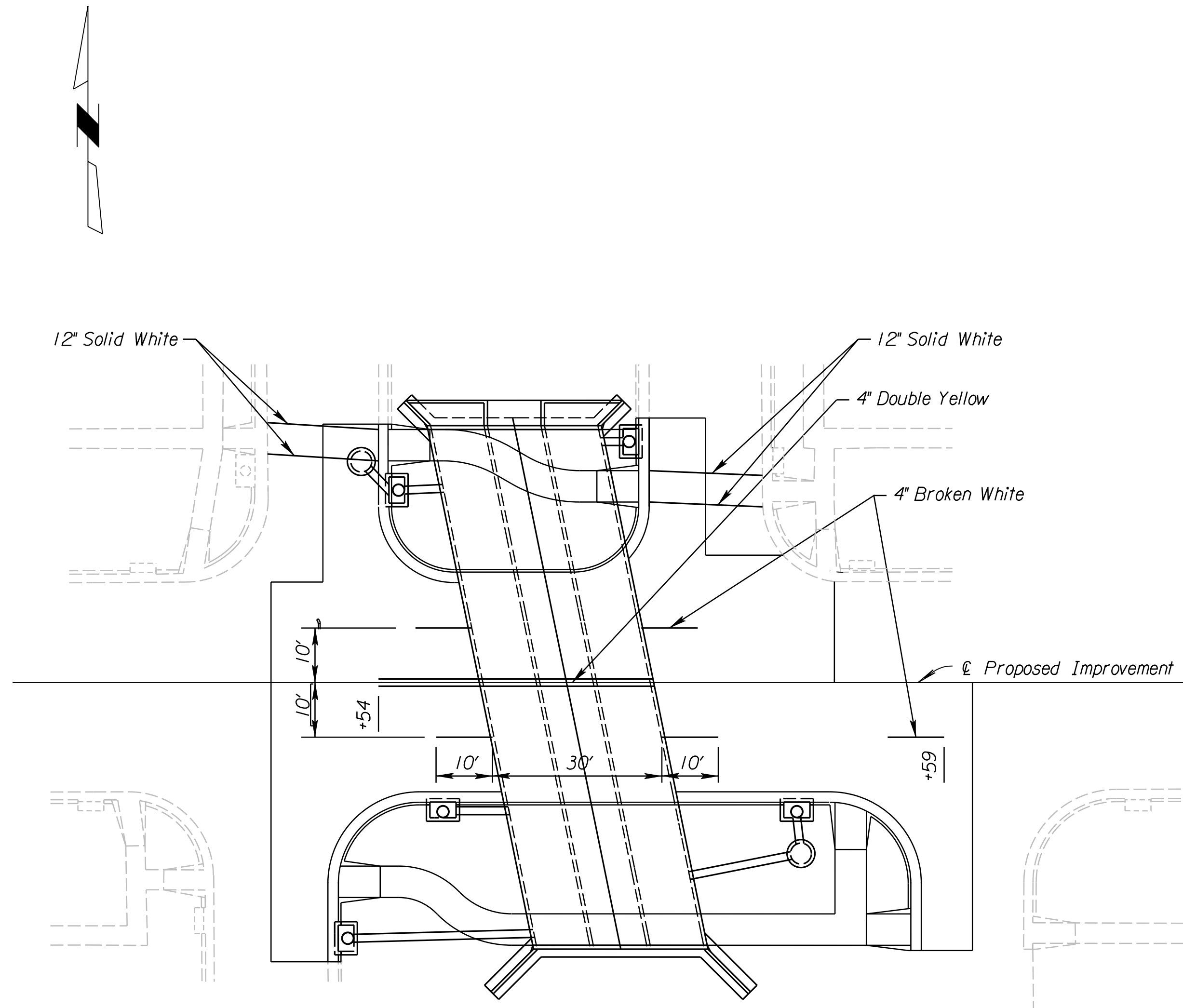
PERMANENT MARKING PLAN
