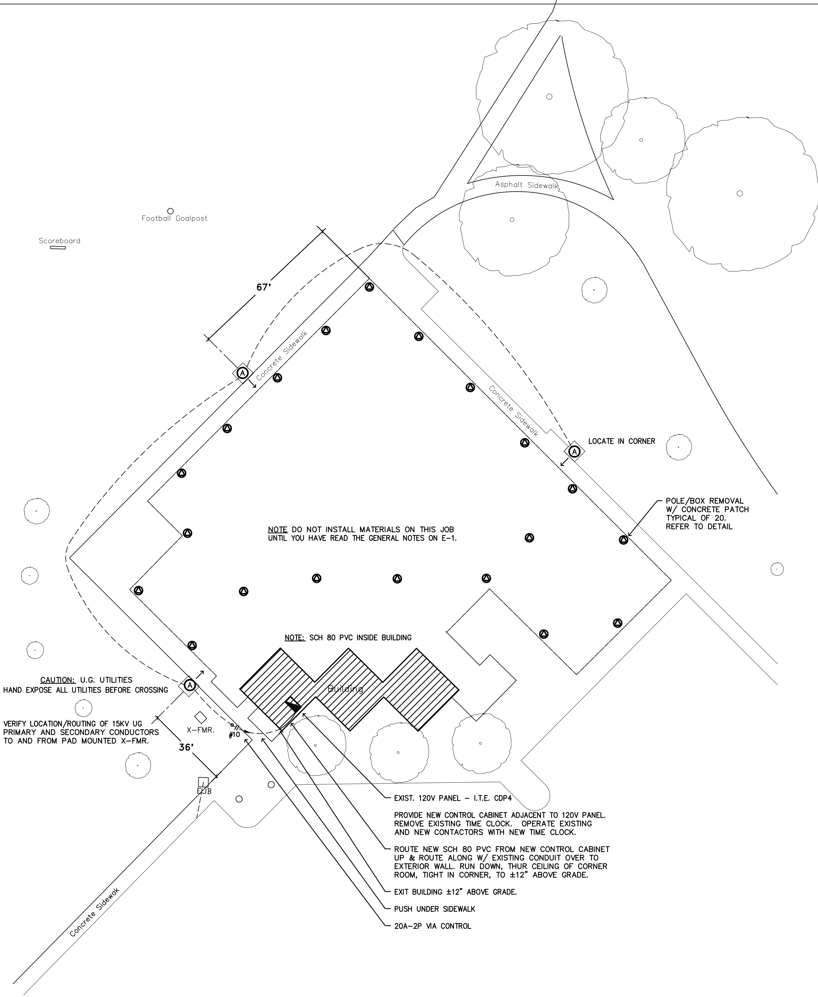
LINWOOD SWIMMING POOL SITE LIGHTING PLAN SCALE: 0 15 30 45 60 75 90
