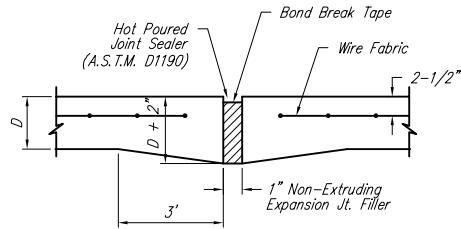
EXPANSION JOINT
