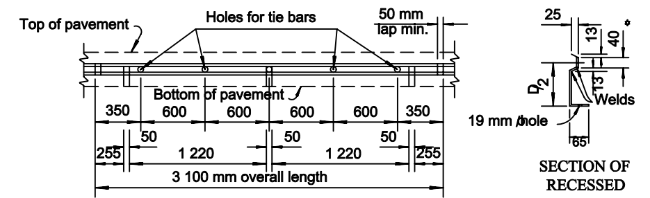
METAL STRIP FOR LONGITUDINAL CONSTRUCTION JOINT
