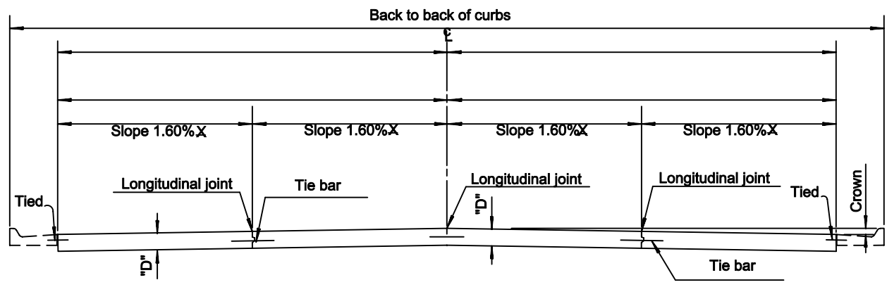
TRANSVERSE SECTION (4 - LANE WITH CURB & GUTTER)
