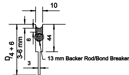
DETAIL OF CONTRACTION JOINT SAWCUT
