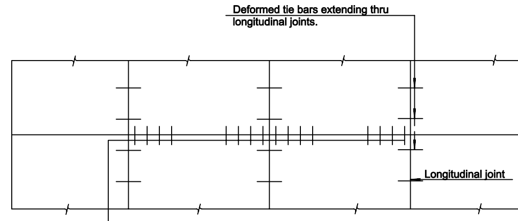
PLAN (2 - LANE WITH SHOULDERS)
