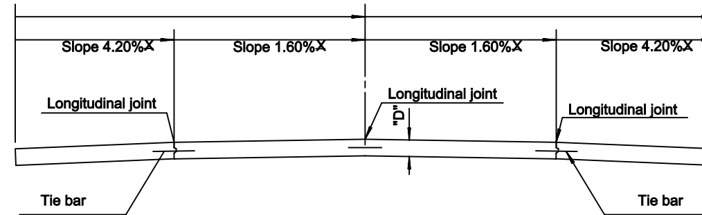
TRANSVERSE SECTION (2 - LANE WITH SHOULDERS)
