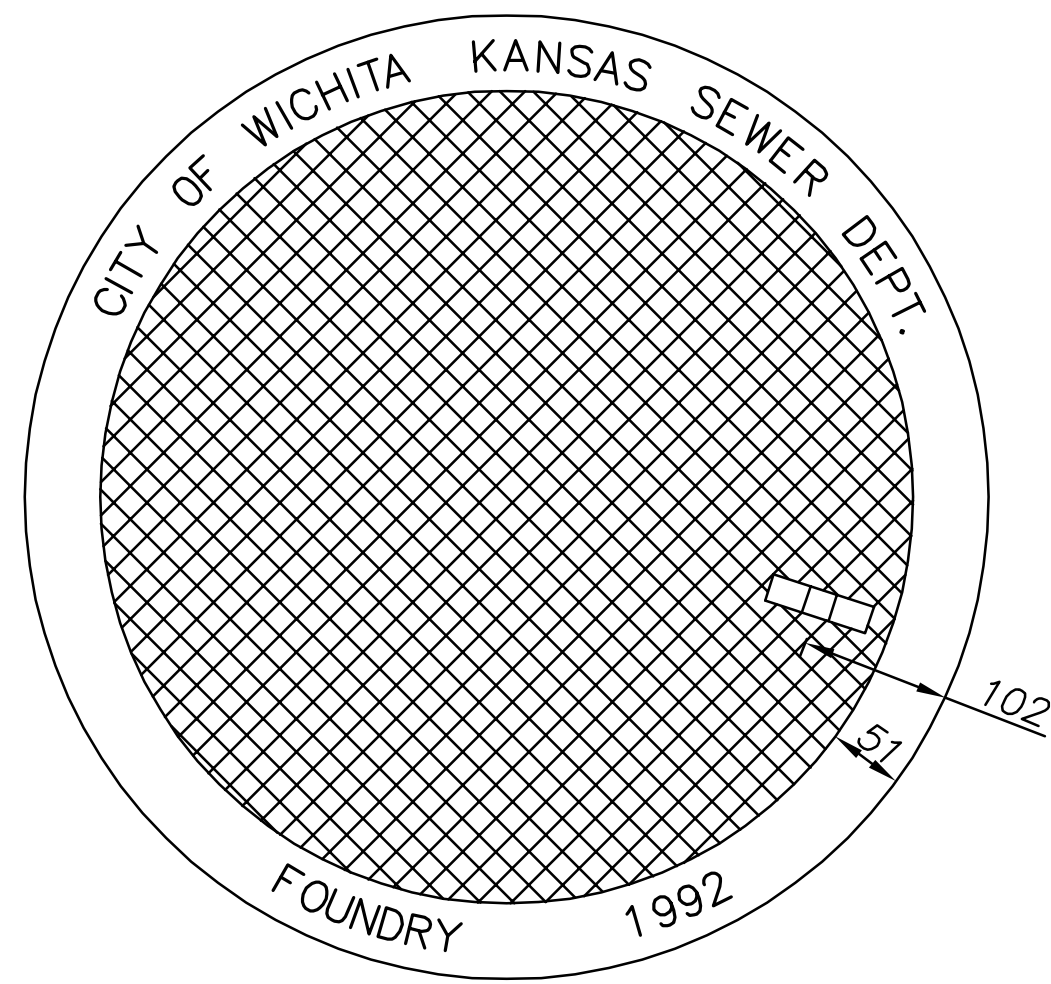
TOP VIEW
