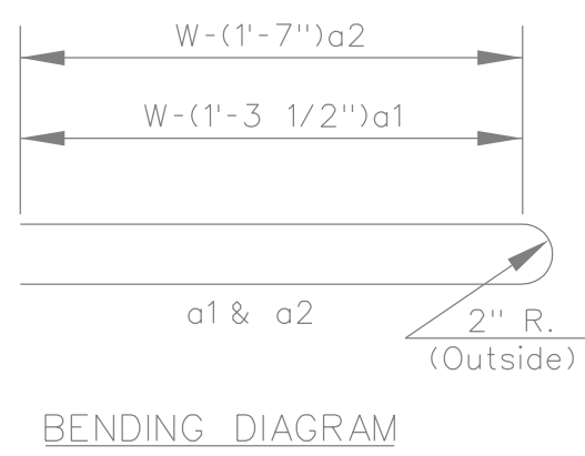
BENDING DIAGRAM
