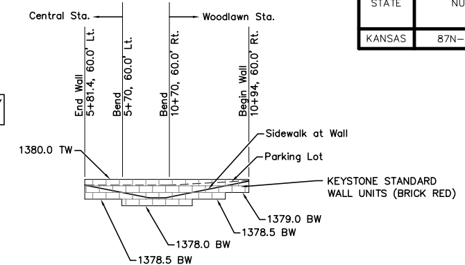
MODULAR BLOCK WALL PROFILE Northeast Corner, See Details Sheet 26.
