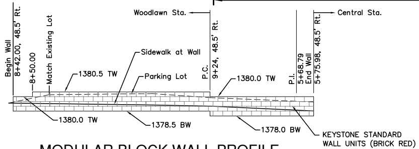
MODULAR BLOCK WALL PROFILE Southeast Corner, See Details Sheet 26.
