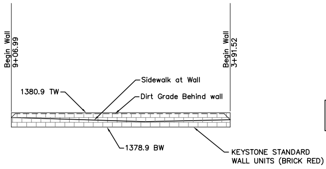
MODULAR BLOCK WALL PROFILE Southwest Corner, See Details Sheet 26.
