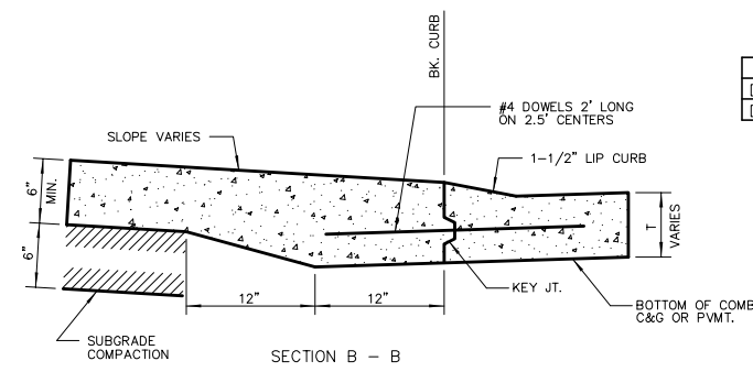
BACK OF CURB DETAIL
