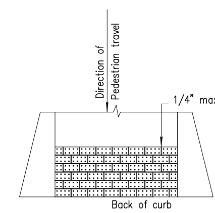
STRAIGHT CURB DETAILS
