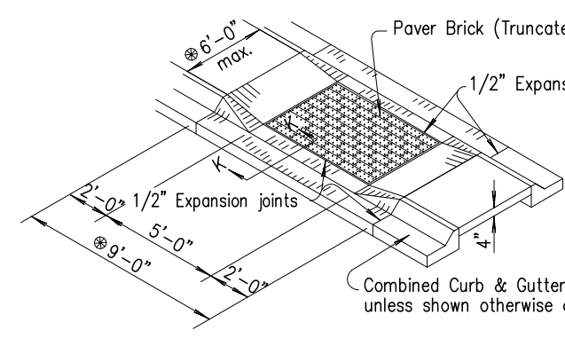
NARROW MEDIAN RAMP CROSSING
