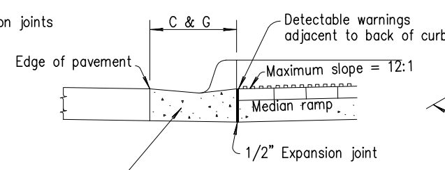
SECTION K-K
