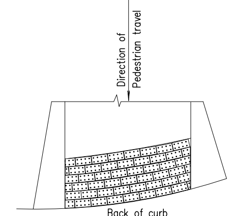
RADIUS CURB DETAILS
