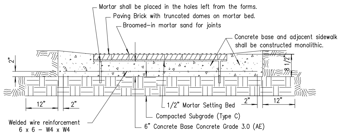
TYPICAL SECTION OF PAVER BRICK SECTION A-A
