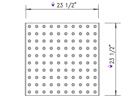
PRESTRESSED RAMP PANEL with TRUNCATED DOME SURFACE
