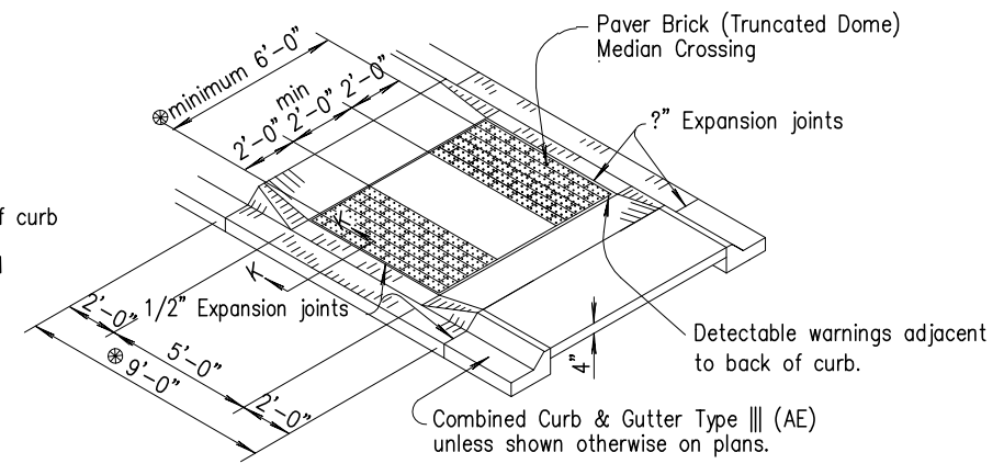
WIDE MEDIAN RAMP CROSSING
