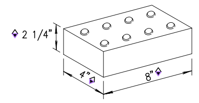
PAVER BRICK WITH TRUNCATED DOME SURFACE
