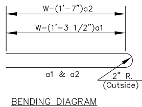
BENDING DIAGRAM
