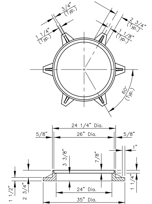
CAST IRON MANHOLE RING
