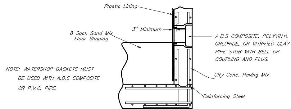
PIPE STUB DETAIL SANITARY SEWER ONLY
