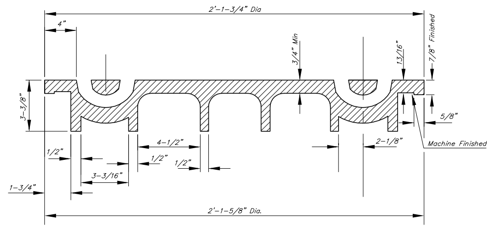
SECTION VIEW
