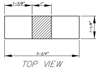
PICKHOLE DETAIL
