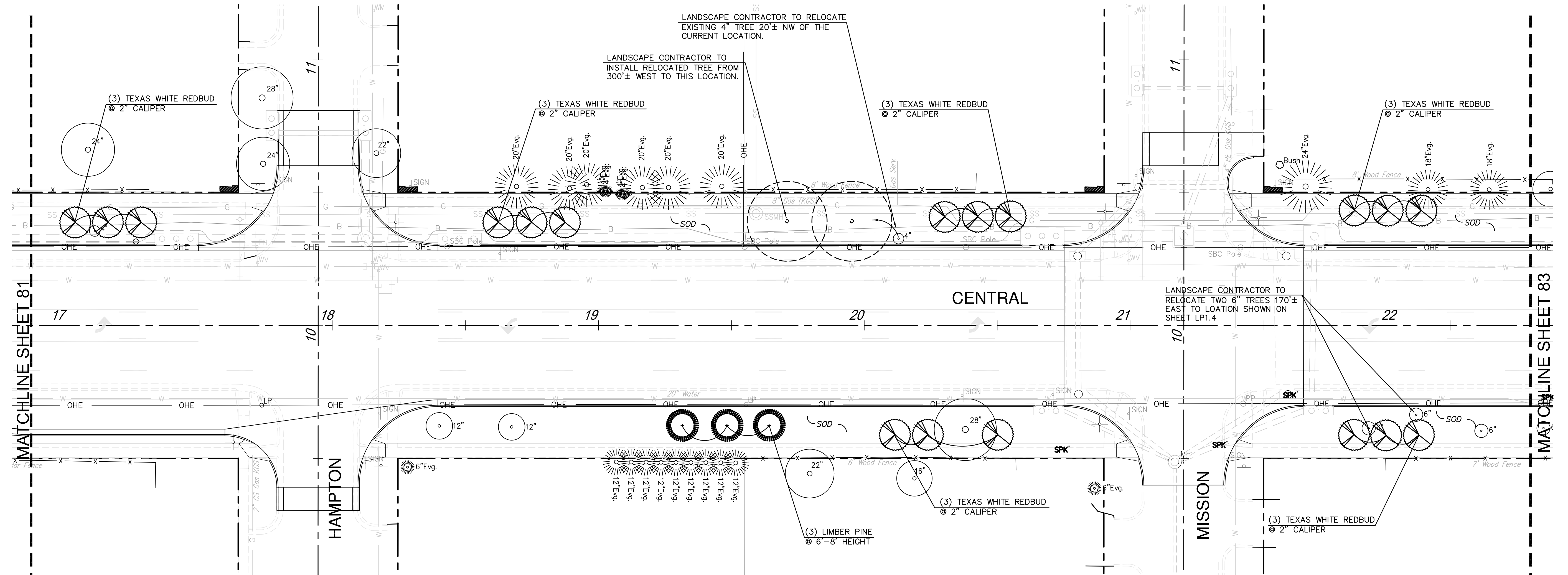
PLANTING PLAN SCALE: 1" = 20'-0"
