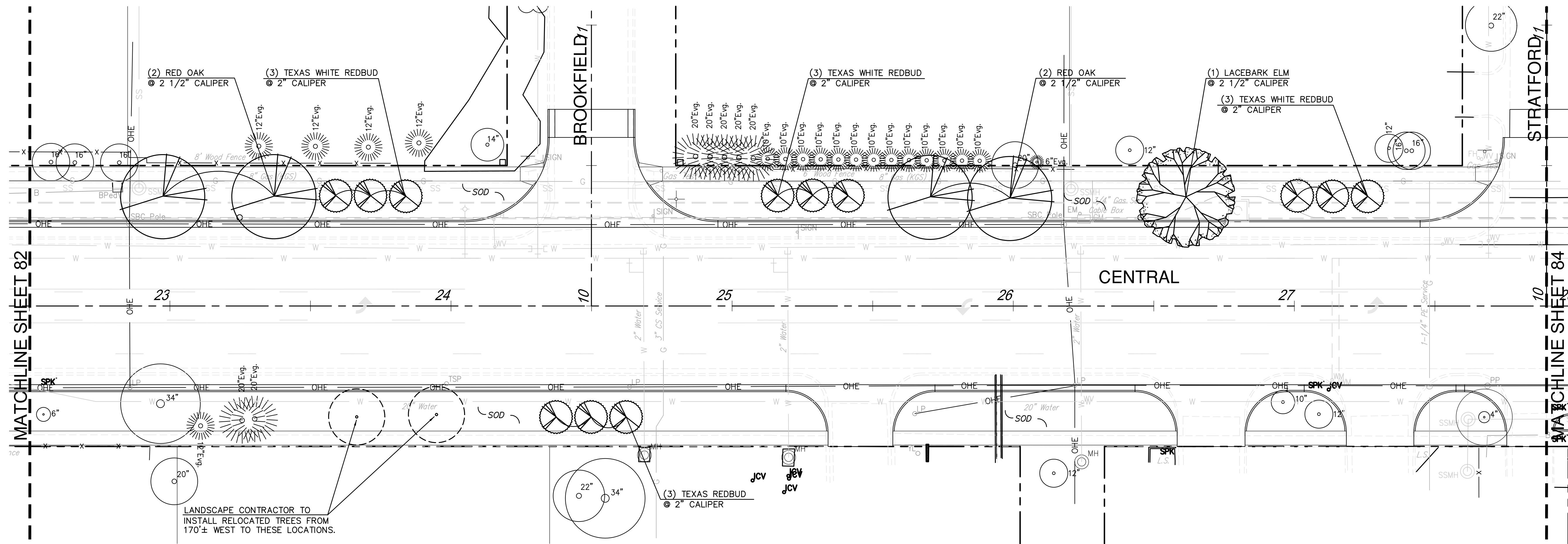
PLANTING PLAN SCALE: 1" = 20'-0"
