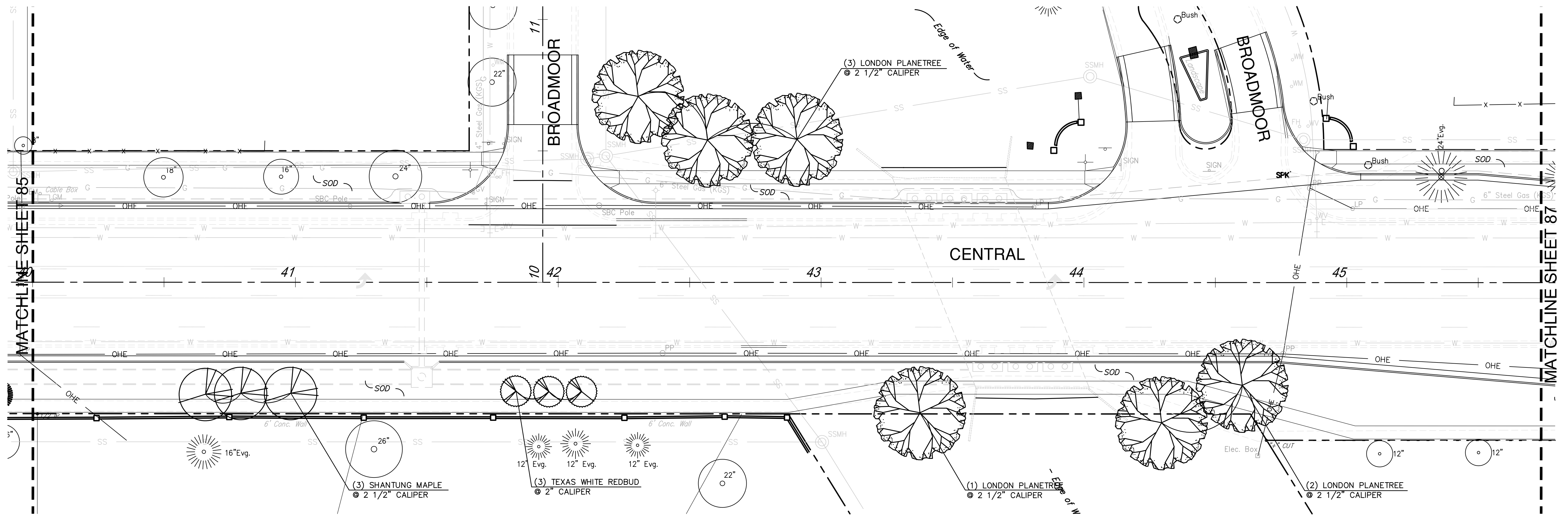
PLANTING PLAN SCALE: 1" = 20'-0"
