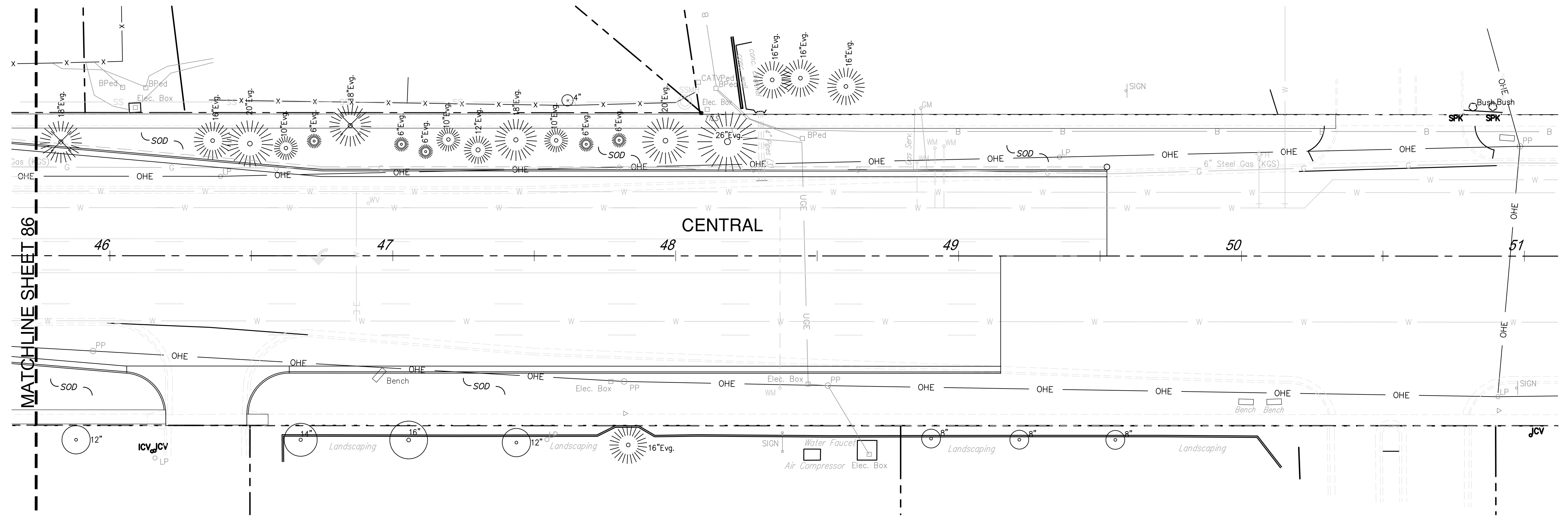
PLANTING PLAN SCALE: 1" = 20'-0"
