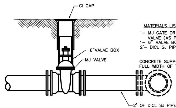
VALVE ASSEMBLY
