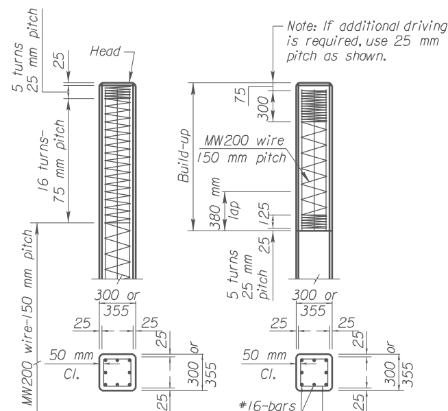
BUILD UP SECTION
