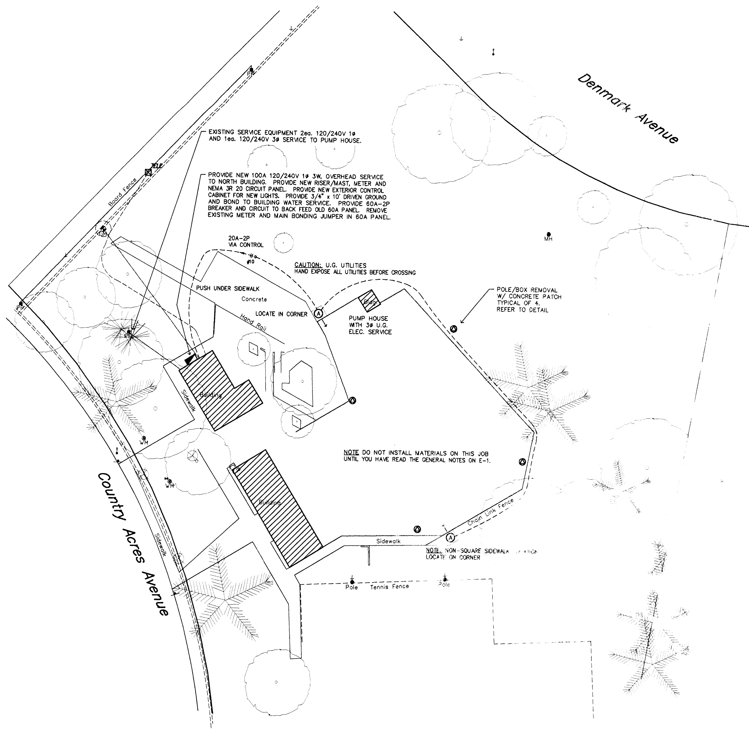
COUNTRY ACRES POOL SITE LIGHTING PLAN
