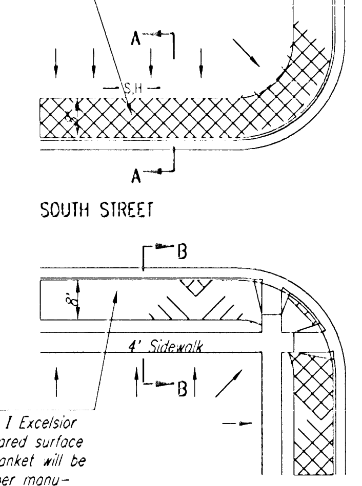
BACK OF CURB PROTECTION DETAIL
